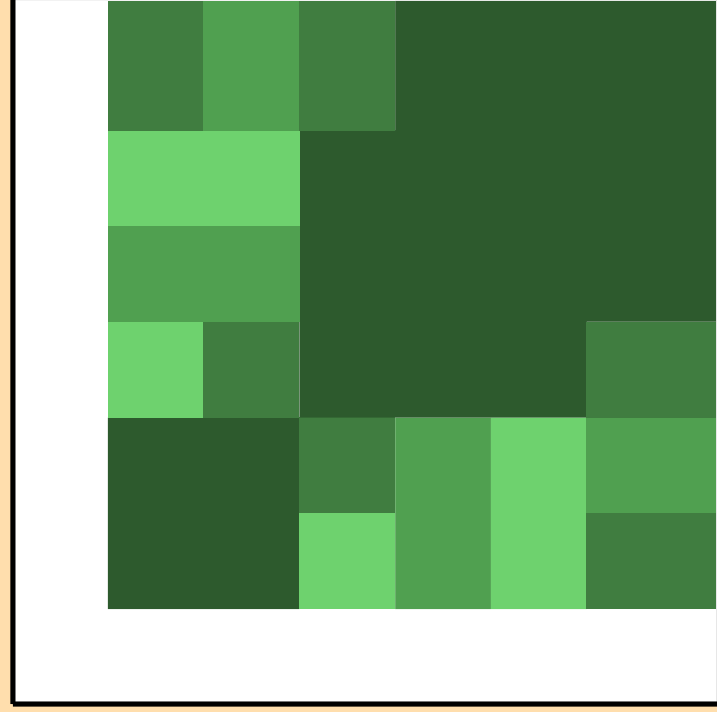
\sigma vs. E for ^{52}\text{Ti}(n,n_1)
