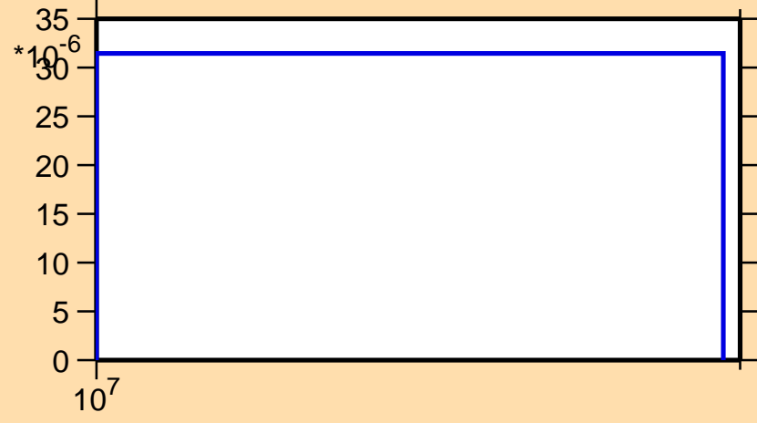
\sigma vs. E for ^{52}\text{Ti}(n,np)
