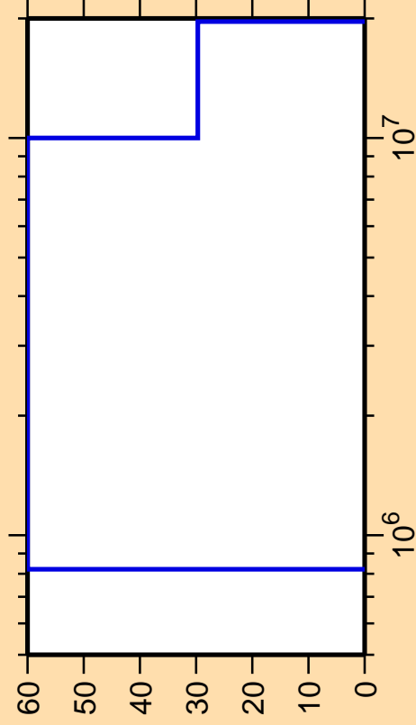
\Delta\sigma/\sigma vs. E for ^{52}\text{Ti}(n,\gamma)
