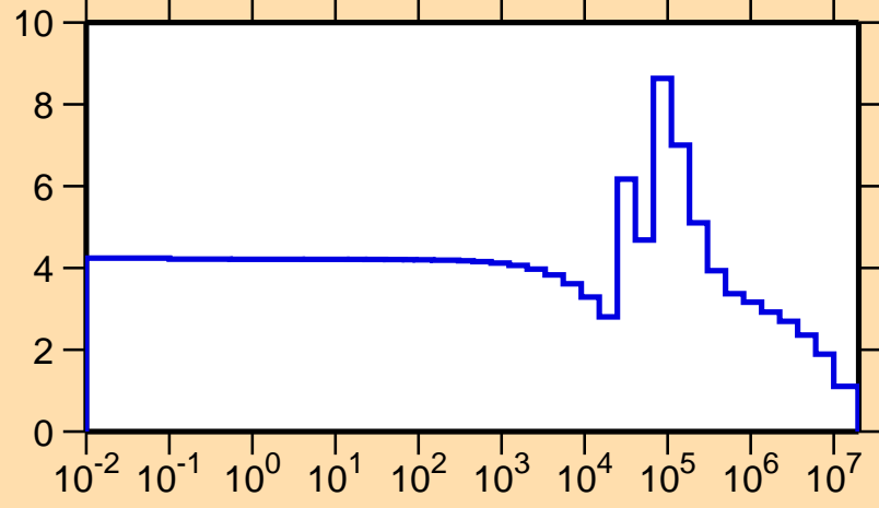
\sigma vs. E for ^{52}\text{Ti}(n,\text{el.})
