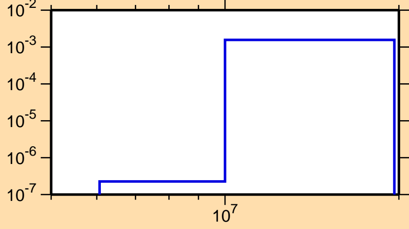
\sigma vs. E for ^{52}\text{Ti}(n,p)
