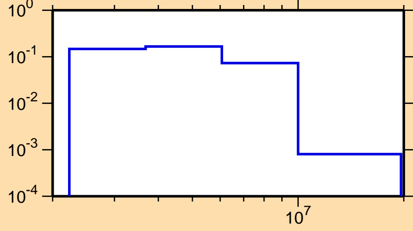
\sigma vs. E for ^{52}\text{Ti}(n,n_4)
