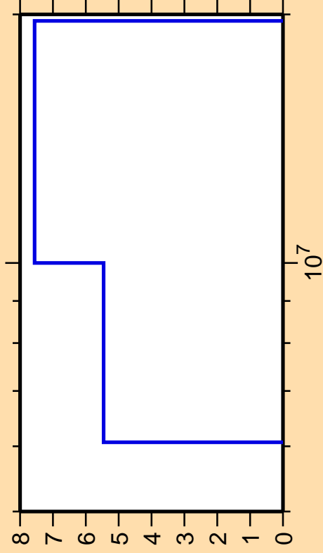
\Delta\sigma/\sigma vs. E for ^{52}\text{Ti}(n,2n)
