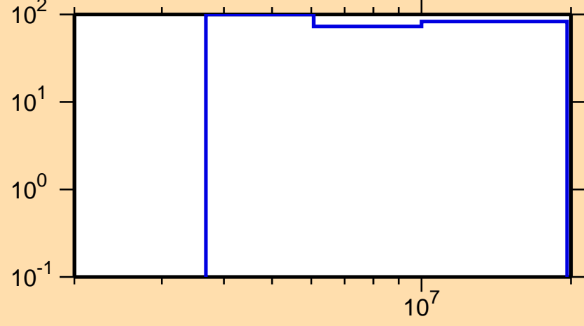
\Delta\sigma/\sigma vs. E for ^{52}\text{Ti}(n,n\text{cont.})
