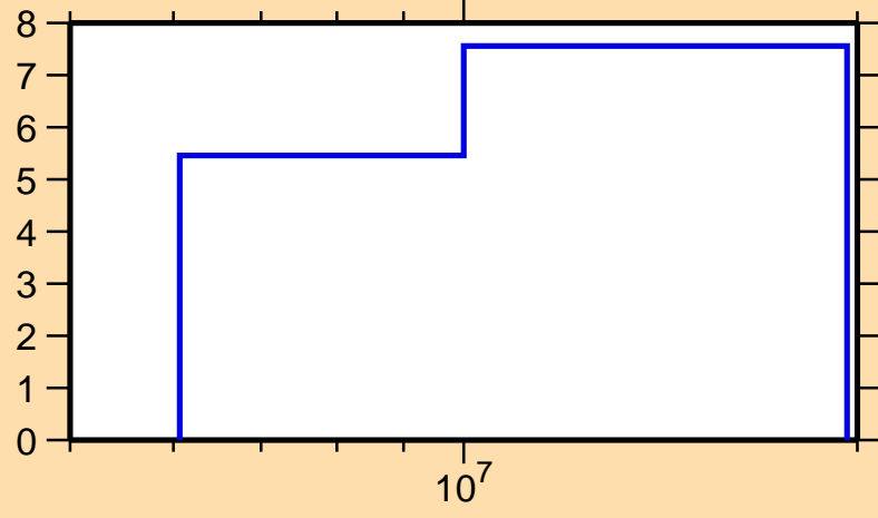
\Delta\sigma/\sigma vs. E for ^{52}\text{Ti}(n,2n)
