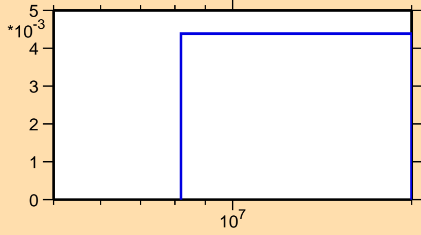
\sigma vs. E for ^{52}\text{Ti}(n,3n)
