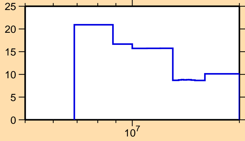
\Delta\sigma/\sigma vs. E for ^{53}\text{Ti}(n,el.)
