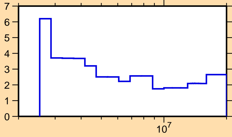
\Delta\sigma/\sigma vs. E for ^{53}\text{Ti}(n,\text{nonel.})
