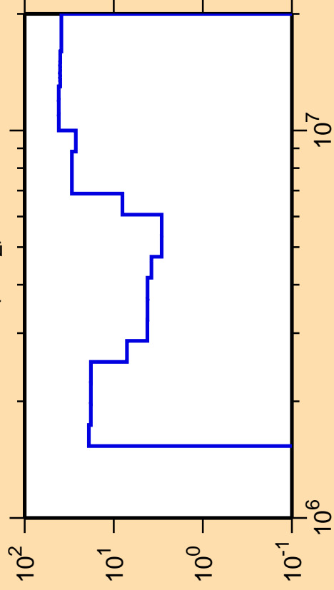
\Delta\sigma/\sigma vs. E for ^{53}\text{Ti}(n,n_2)
