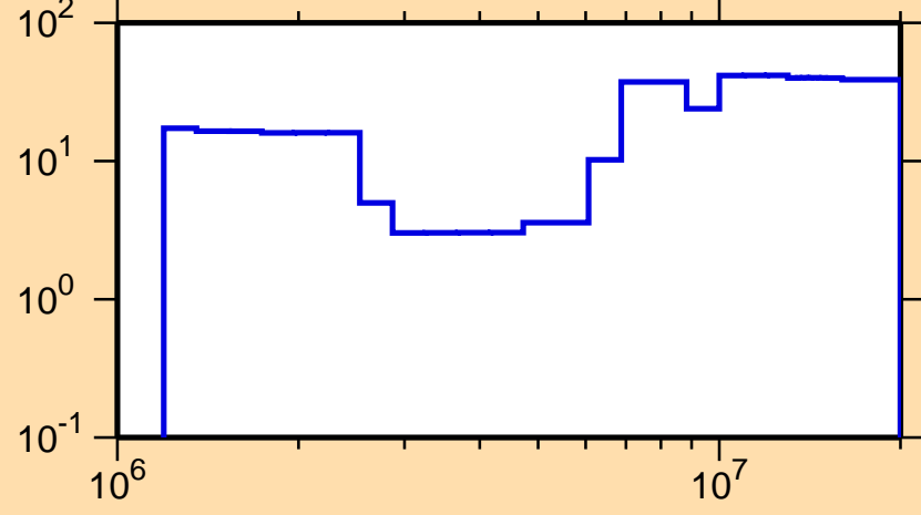
\Delta\sigma/\sigma vs. E for ^{53}\text{Ti}(n,n_1)
