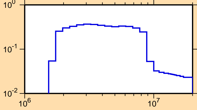
\sigma vs. E for ^{53}\text{Ti}(n,n_2)
