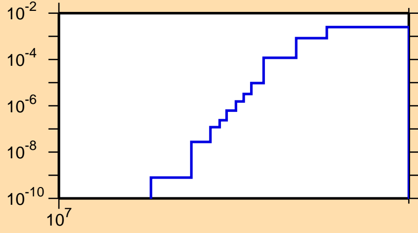
\sigma vs. E for ^{53}\text{Ti}(n,d)
