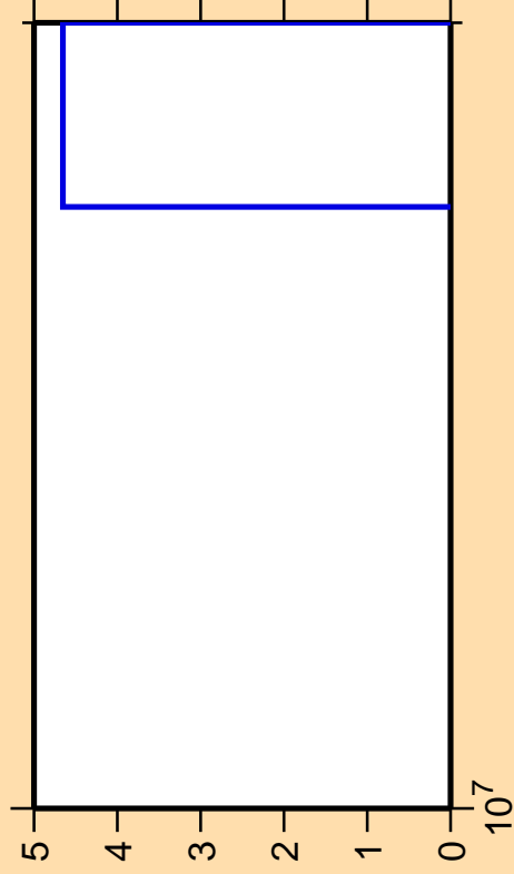
\Delta\sigma/\sigma vs. E for ^{53}\text{Ti}(n,2np)
