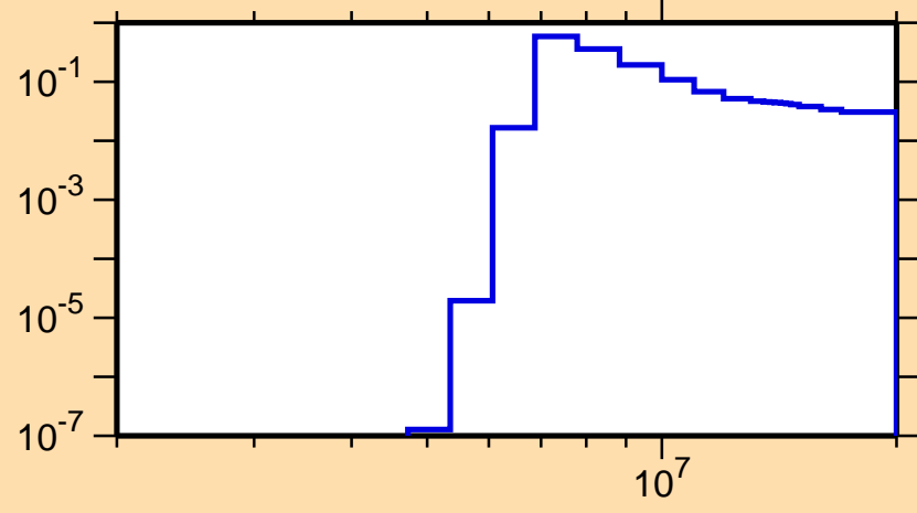
\sigma vs. E for ^{54}\text{Ti}(n,n\text{cont.})
