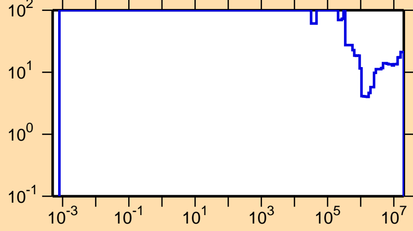
\Delta\sigma/\sigma vs. E for ^{54}\text{Ti}(n,\text{tot.})
