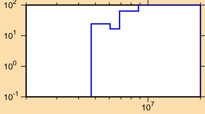
\Delta\sigma/\sigma vs. E for ^{54}\text{Ti}(n,\text{inel.})
