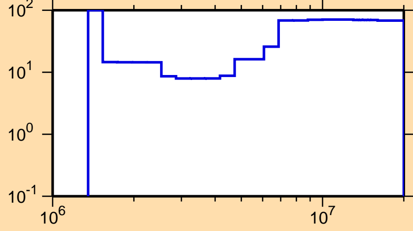
\Delta\sigma/\sigma vs. E for ^{54}\text{Ti}(n,n_1)
