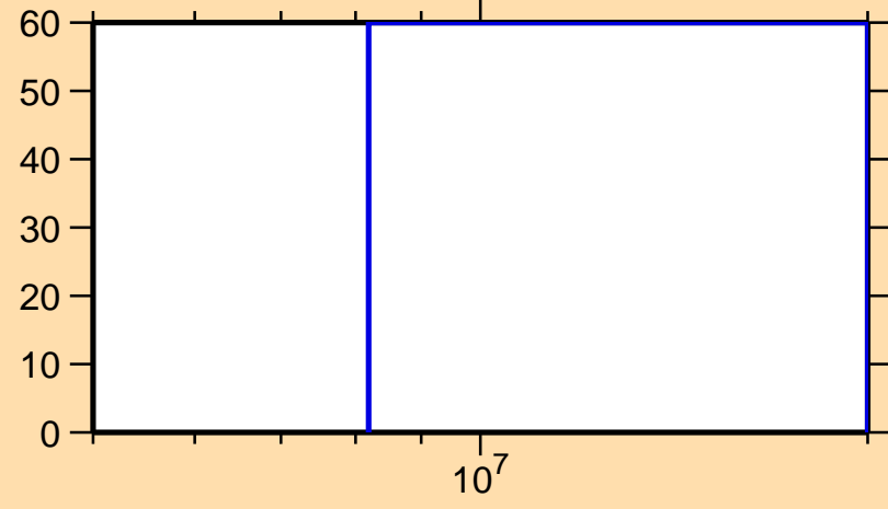
\Delta\sigma/\sigma vs. E for ^{54}\text{Ti}(n,ncont.)
