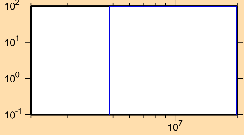
\Delta\sigma/\sigma vs. E for ^{54}\text{Ti}(n,n\text{cont.})
