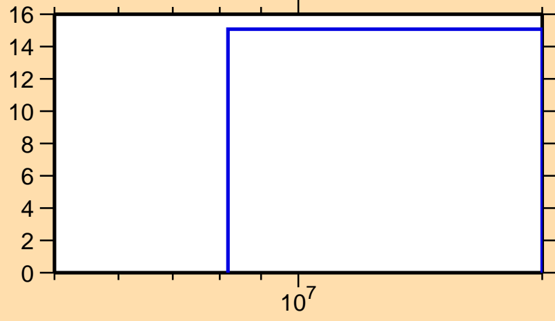
\Delta\sigma/\sigma vs. E for ^{54}\text{Ti}(n,el.)
