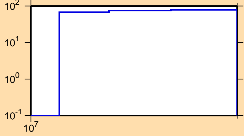
\Delta\sigma/\sigma vs. E for ^{55}\text{Ti}(n,p)
