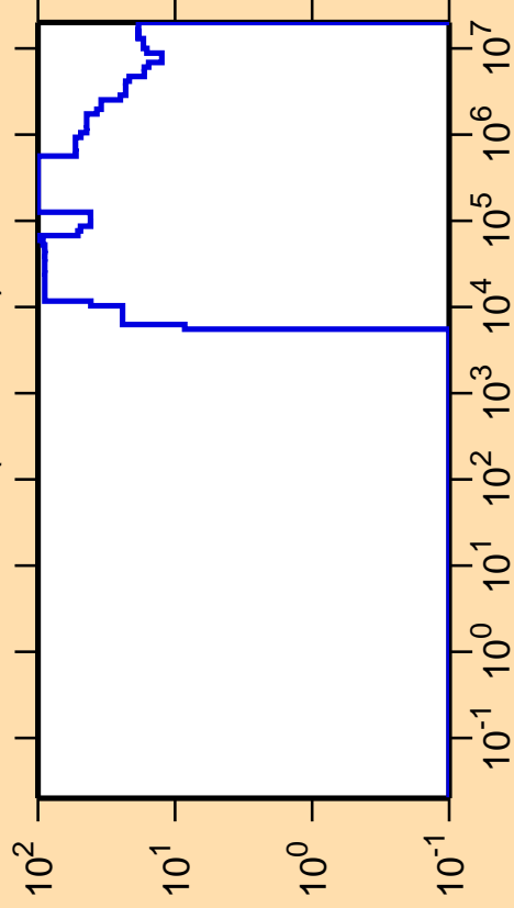
\Delta\sigma/\sigma vs. E for ^{55}\text{Ti}(n,\text{nonel.})
