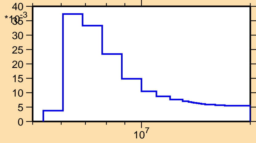
\sigma vs. E for ^{55}\text{Ti}(n,n\text{cont.})
