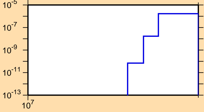
\sigma vs. E for ^{55}\text{Ti}(n,2n\alpha)
