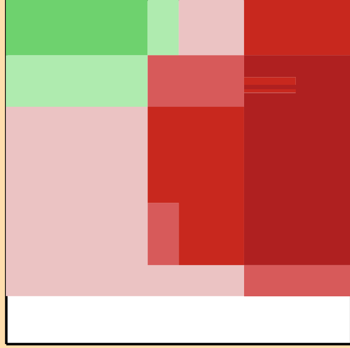
\Delta\sigma/\sigma vs. E for ^{55}\text{Ti}(n,n_1)
