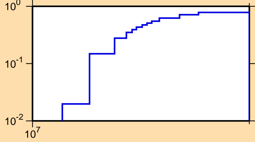
\sigma vs. E for ^{55}\text{Ti}(n,3n)
