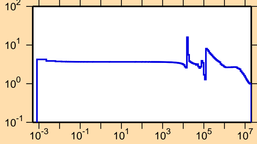
\sigma vs. E for ^{55}\text{Ti}(n,\text{el.})
