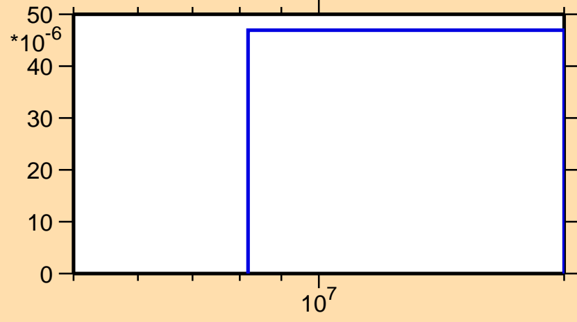
\sigma vs. E for ^{55}\text{Ti}(n,t)
