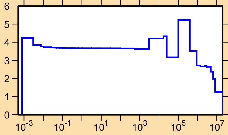
\sigma vs. E for ^{55}\text{Ti}(n,\text{el.})
