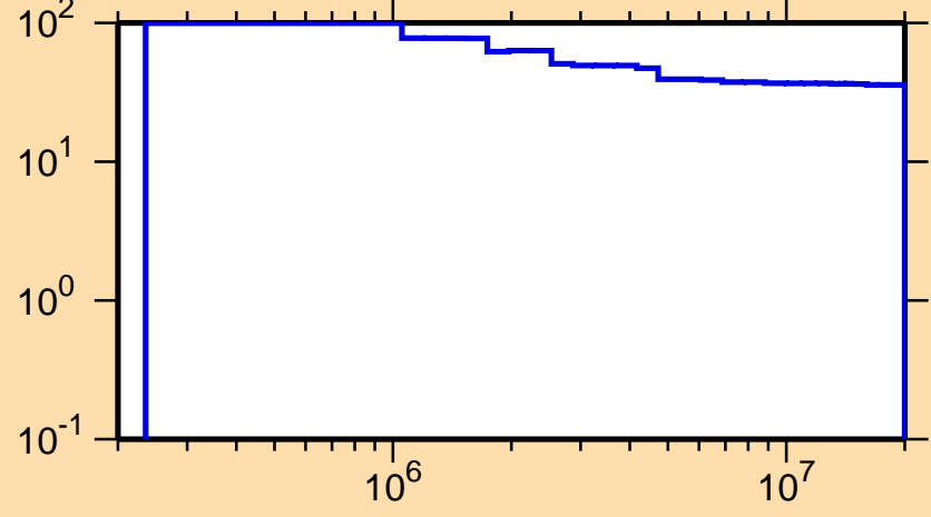
\Delta\sigma/\sigma vs. E for ^{181}\text{Tl}(n,n_1)
