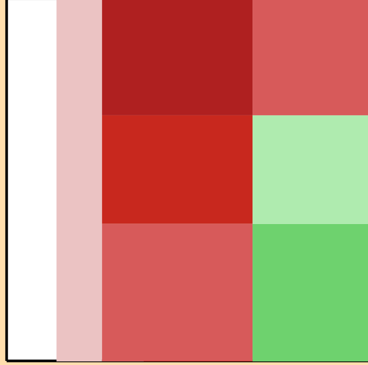
\Delta\sigma/\sigma vs. E for ^{181}\text{Tl}(n,2n)
