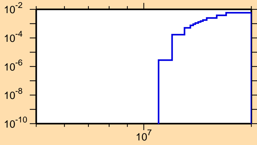
\sigma vs. E for ^{181}\text{Tl}(n,2n\alpha)
