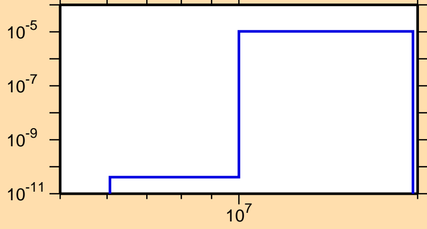
\sigma vs. E for ^{181}\text{Tl}(n,\text{pd})
