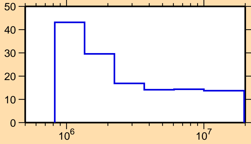
\Delta\sigma/\sigma vs. E for ^{181}\text{Tl}(n,n\text{nonel.})
