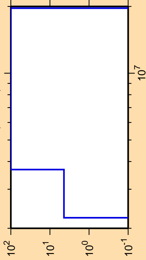
\Delta\sigma/\sigma vs. E for ^{181}\text{Tl}(n,\text{He3})
