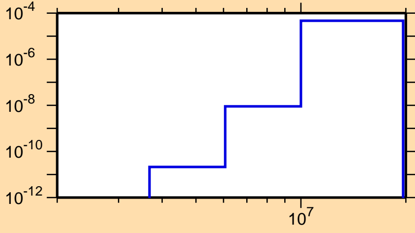
\sigma vs. E for ^{181}\text{Tl}(n,\text{He3})
