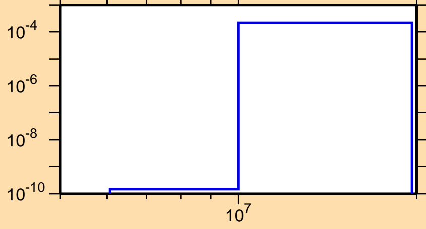
\sigma vs. E for ^{181}\text{Tl}(n,t)
