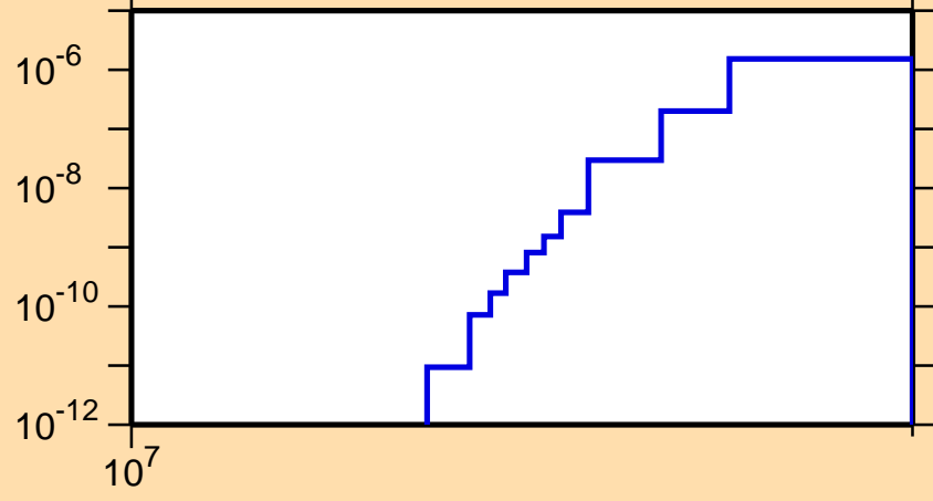
\sigma vs. E for ^{183}\text{Tl}(n,\text{nd})
