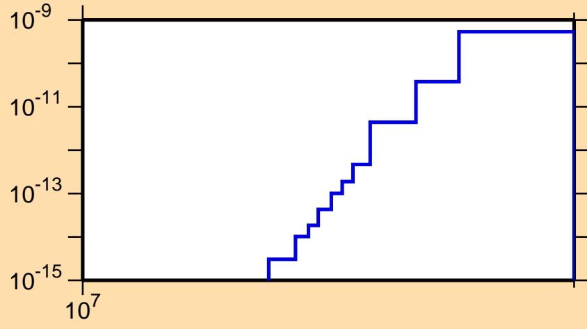
\sigma vs. E for ^{183}\text{Tl} (mt 34)
