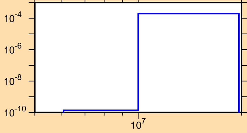
\sigma vs. E for ^{183}\text{Tl}(n,t)
