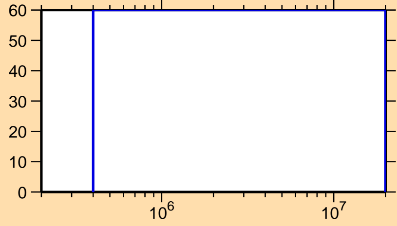
\Delta\sigma/\sigma vs. E for ^{183}\text{Tl}(n,n\text{cont.})
