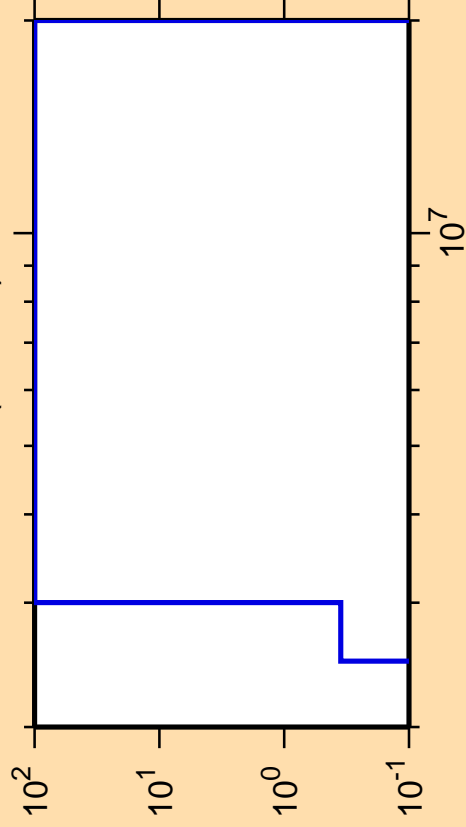
\Delta\sigma/\sigma vs. E for ^{183}\text{Tl}(\text{mt117})
