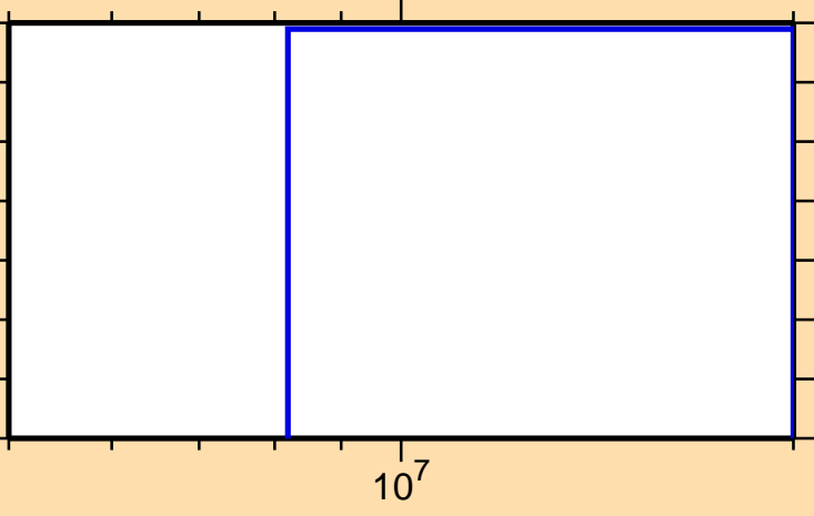
\sigma vs. E for ^{183}\text{Tl}(n,2n\alpha)
