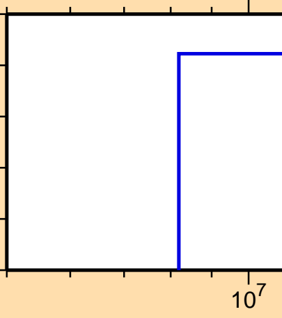
\sigma vs. E for ^{183}\text{Tl}(n,\text{pd})
