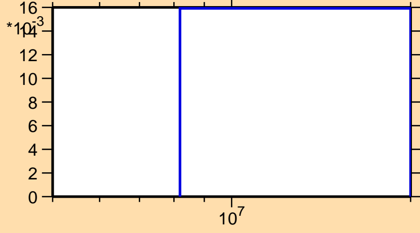
\sigma vs. E for ^{183}\text{Tl}(n,2n)
