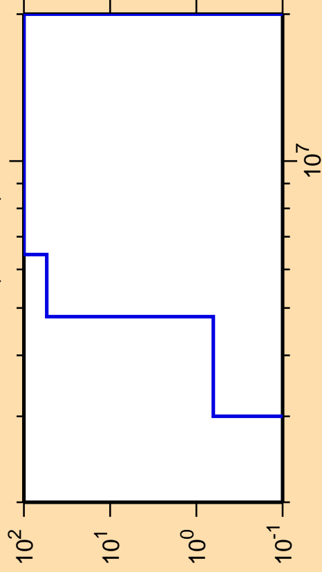
\Delta\sigma/\sigma vs. E for ^{183}\text{Tl}(n,\text{He3})
