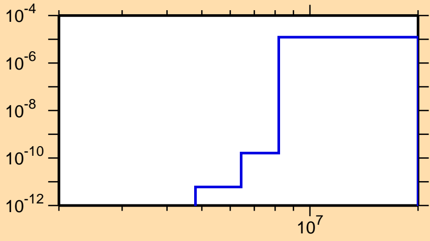
\sigma vs. E for ^{183}\text{Tl}(n,\text{He3})
