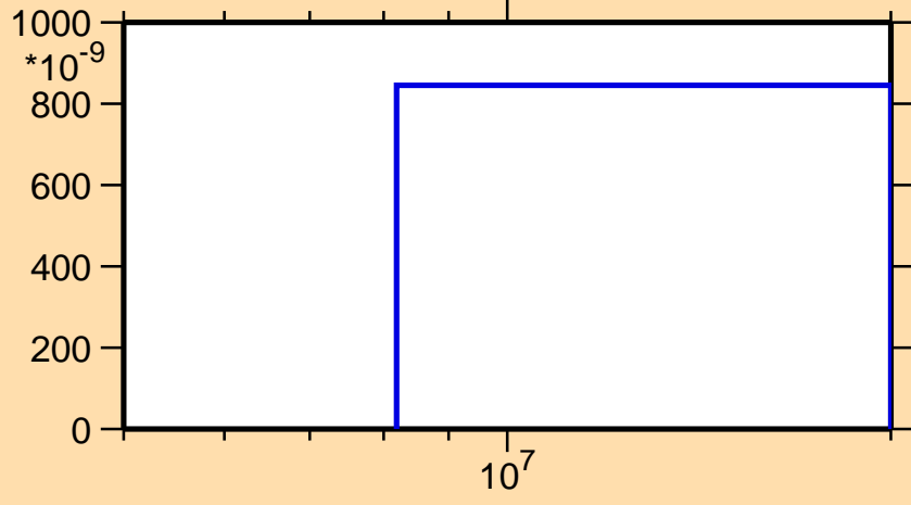
\sigma vs. E for ^{183}\text{Tl}(n,\text{pd})
