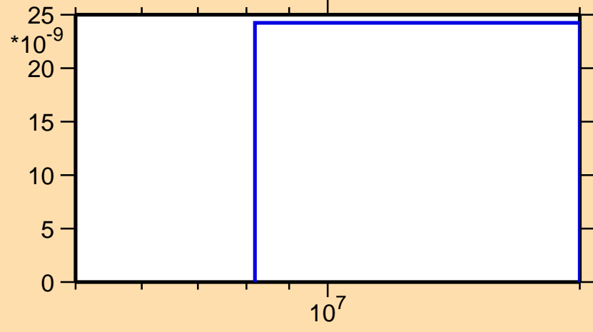
\sigma vs. E for ^{183}\text{Tl}(n,\text{nd})
