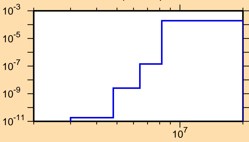
\sigma vs. E for ^{183}\text{Tl}(\text{mt117})
