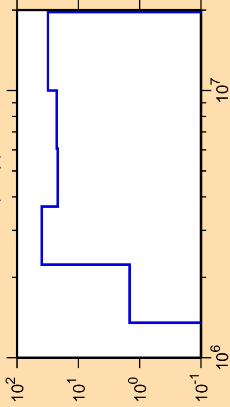
\Delta\sigma/\sigma vs. E for ^{184}\text{Tl}(n,np)
