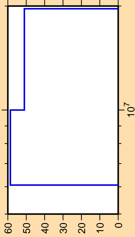
\Delta\sigma/\sigma vs. E for ^{184}\text{Tl}(n,n_1)
