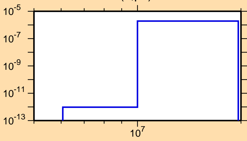
\sigma vs. E for ^{184}\text{Tl}(n,\text{pd})
