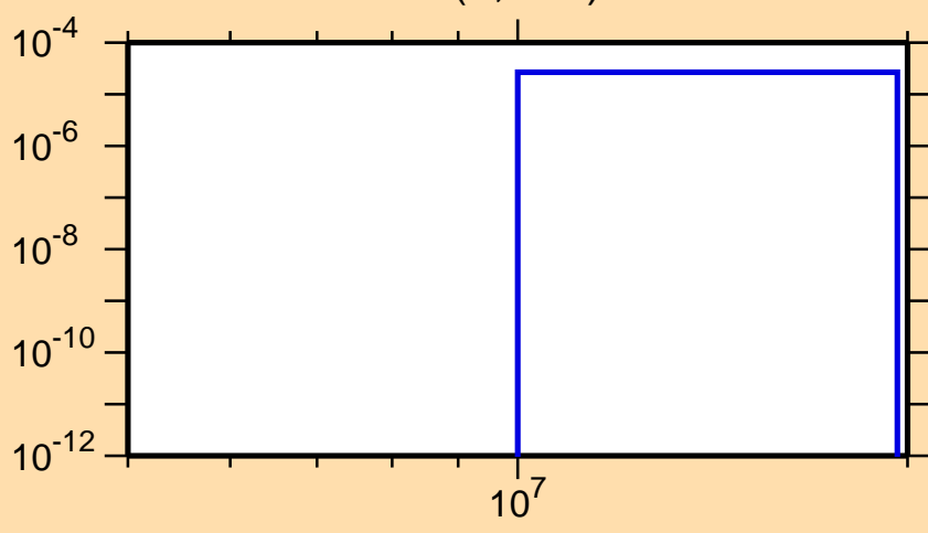
\sigma vs. E for ^{184}\text{Tl}(n,2n\alpha)
