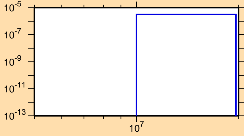
\sigma vs. E for ^{184}\text{Tl}(n,\text{nd})
