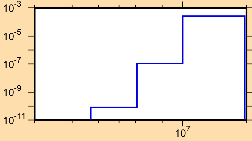
\sigma vs. E for ^{184}\text{Tl} (mt 45)
