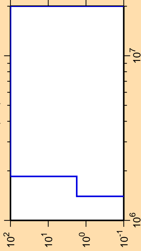
\Delta\sigma/\sigma vs. E for ^{184}\text{Tl}(n,d)
