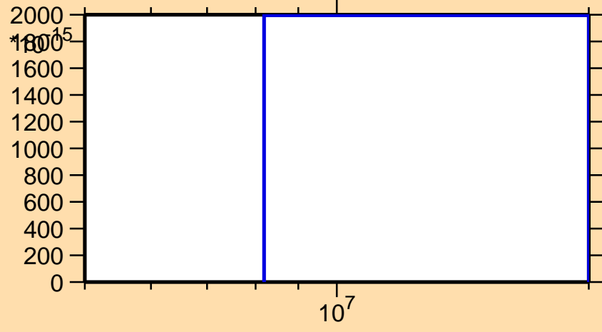
\sigma vs. E for ^{184}\text{Tl}(n,3n)
