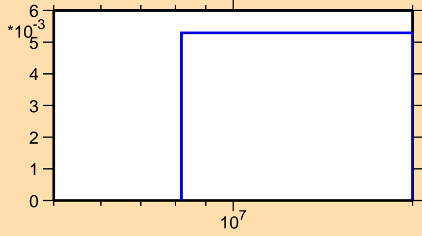
\sigma vs. E for ^{184}\text{Tl}(n,2np)
