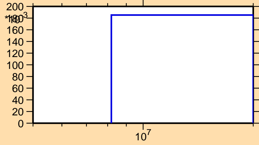
\sigma vs. E for ^{184}\text{Tl}(n,2n)
