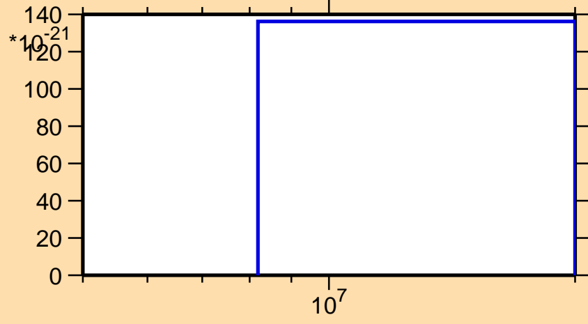
\sigma vs. E for ^{184}\text{Tl} (mt 42)
