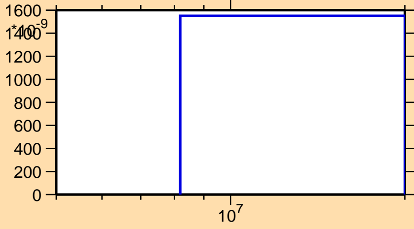
\sigma vs. E for ^{184}\text{Tl}(n,\text{pd})
