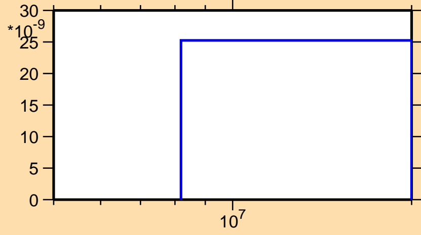
\sigma vs. E for ^{184}\text{Tl}(n,\text{pt})
