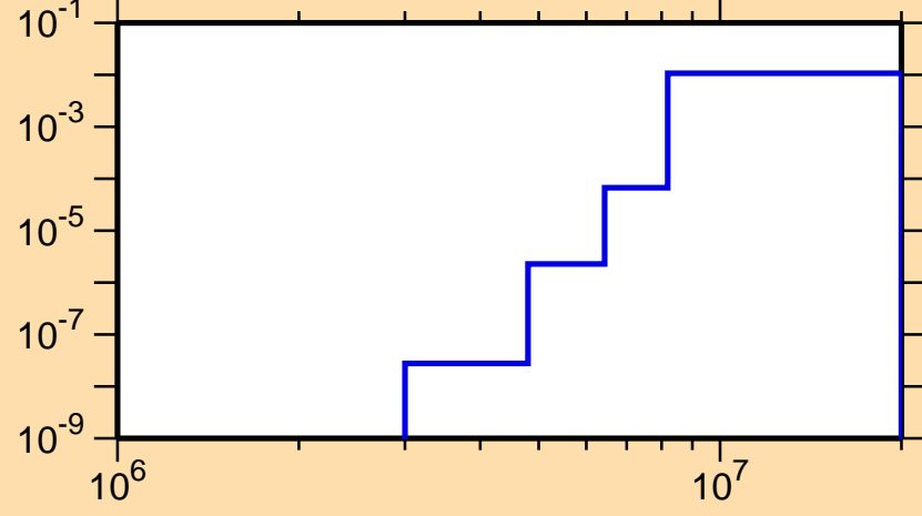
\sigma vs. E for ^{184}\text{Tl}(n,d)
