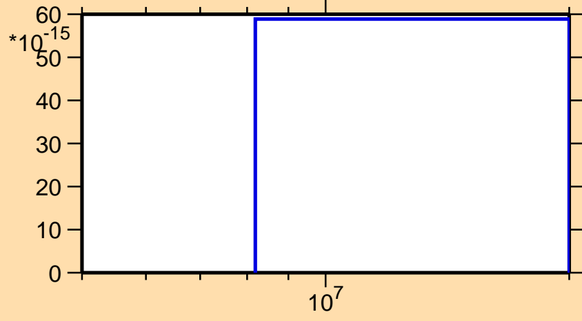
\sigma vs. E for ^{184}\text{Tl}(n,3n\alpha)
