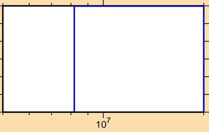
\sigma vs. E for ^{185}\text{Tl}(n,3n)
