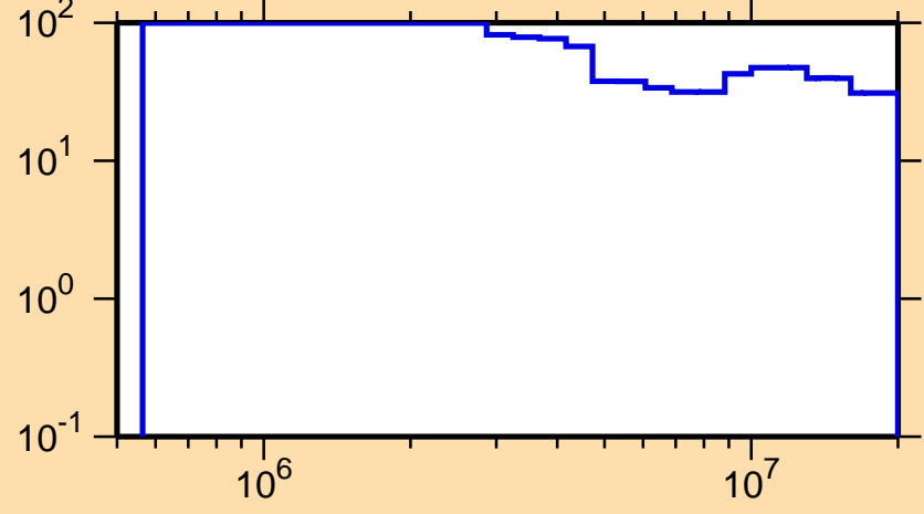
\Delta\sigma/\sigma vs. E for ^{186}\text{Tl}(n,n\text{cont.})
