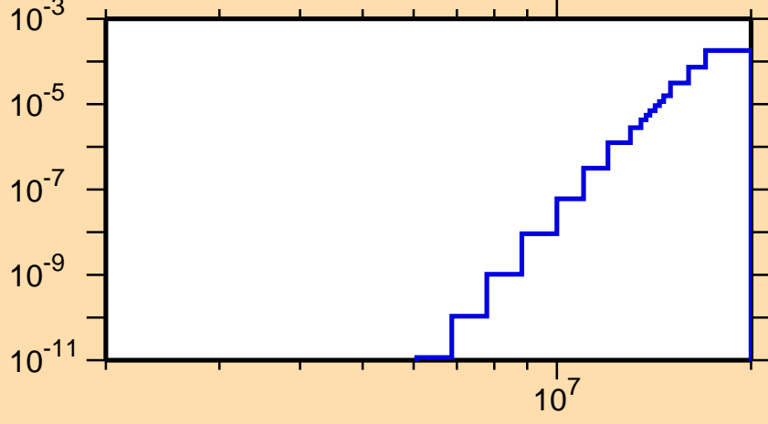
\sigma vs. E for ^{186}\text{Tl}(n,\text{He3})
