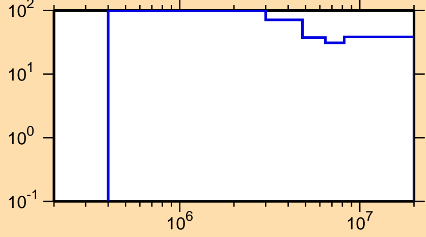
\Delta\sigma/\sigma vs. E for ^{186}\text{Tl}(n,ncont.)
