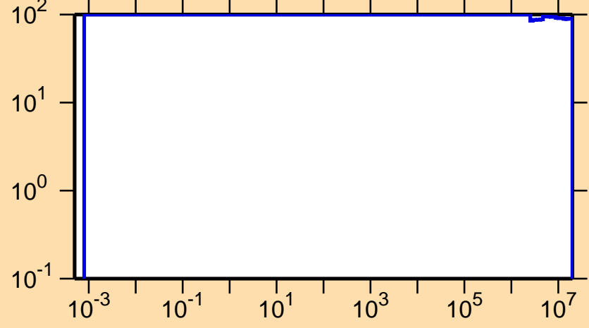
\Delta\sigma/\sigma vs. E for ^{186}\text{Tl}(n,p)
