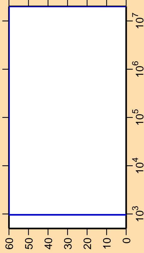
\Delta\sigma/\sigma vs. E for ^{186}\text{Tl}(n,n\text{cont.})
