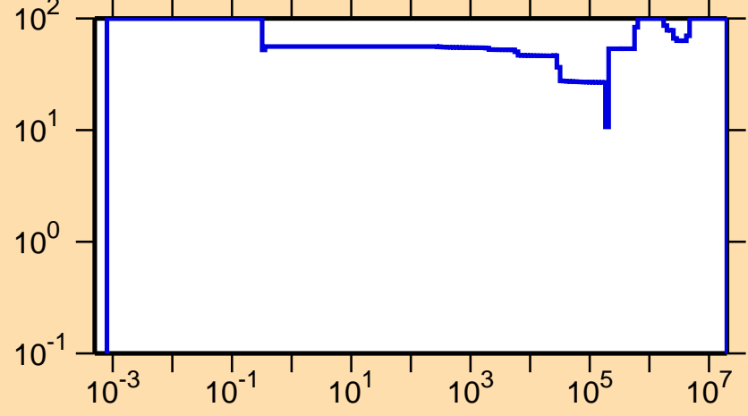
\Delta\sigma/\sigma vs. E for ^{186}\text{Tl}(n,\text{el.})
