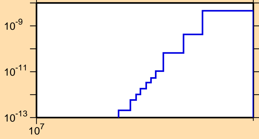
\sigma vs. E for ^{186}\text{Tl}(\text{mt } 34)
