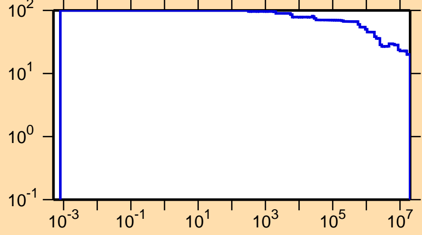
\Delta\sigma/\sigma vs. E for ^{186}\text{Tl}(n,\text{nonel.})
