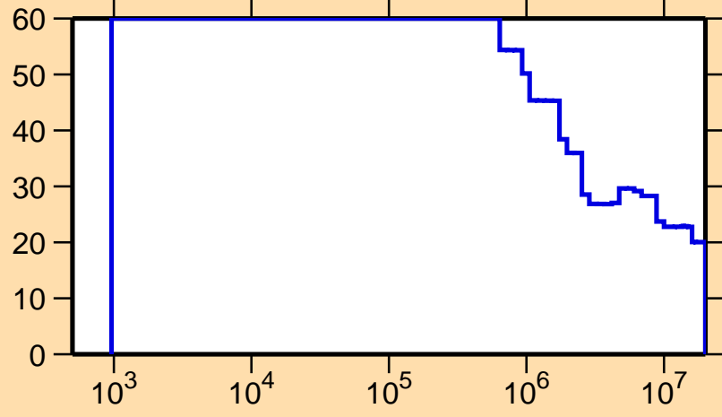
\Delta\sigma/\sigma vs. E for ^{186}\text{Tl}(n,n\text{nonel.})
