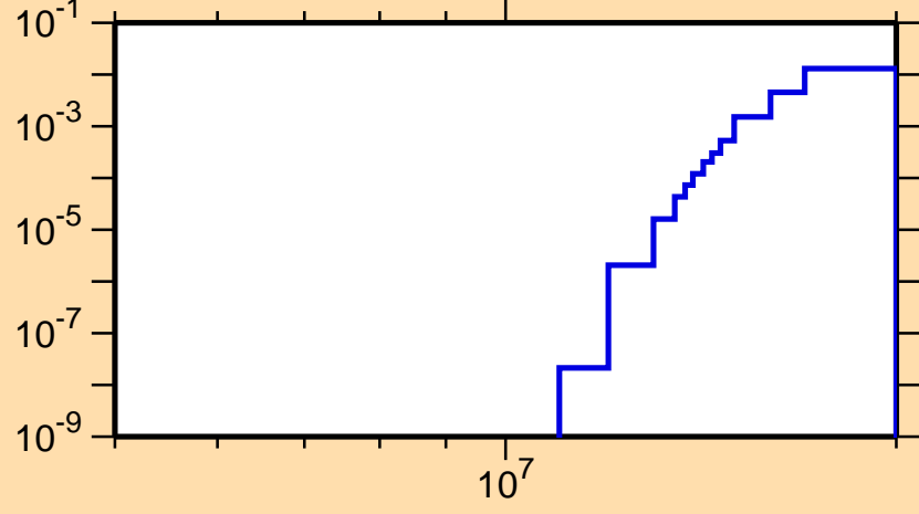
\sigma vs. E for ^{186}\text{Tl}(n,2np)
