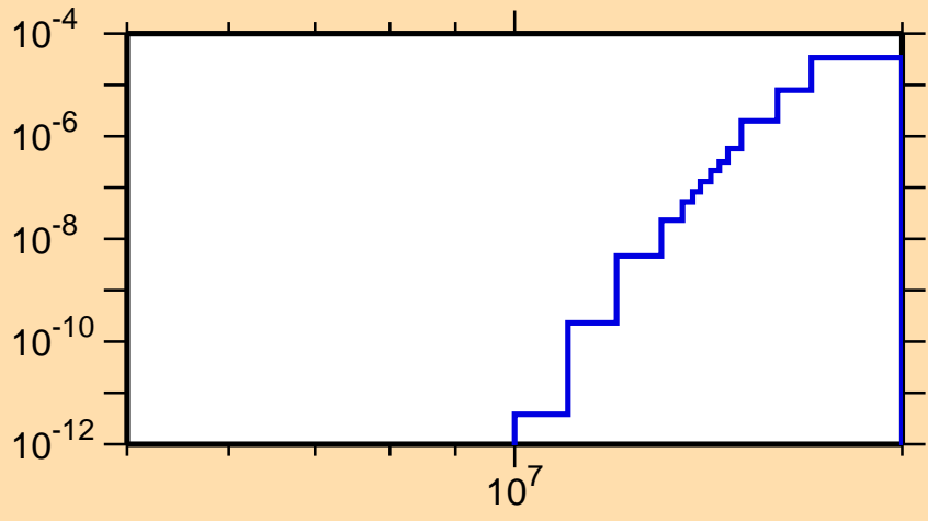
\sigma vs. E for ^{186}\text{Tl}(n,\text{nd})
