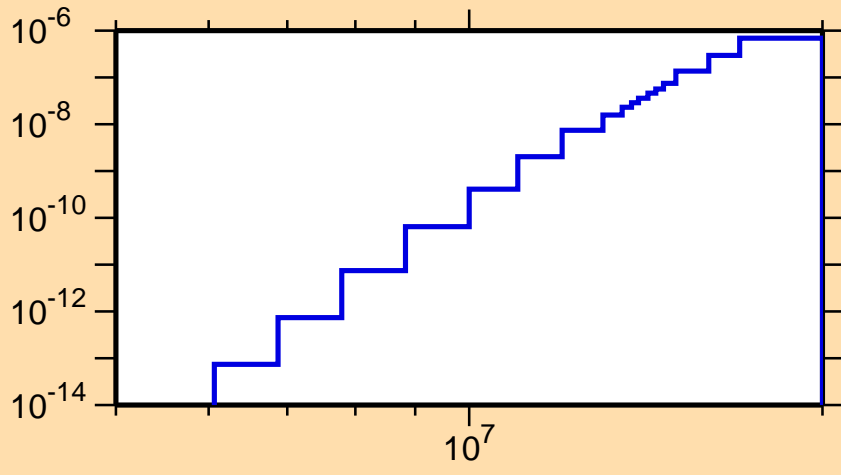
\sigma vs. E for ^{186}\text{Tl}(\text{mt117})
