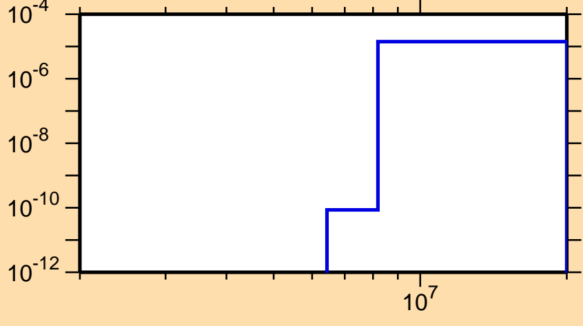
\sigma vs. E for ^{186}\text{Tl} (mt 45)
