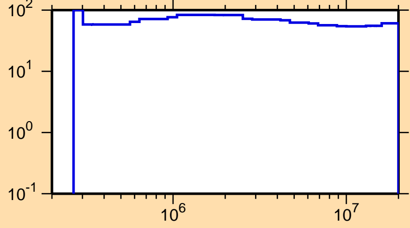
\Delta\sigma/\sigma vs. E for ^{187}\text{Tl}(n,ncont.)
