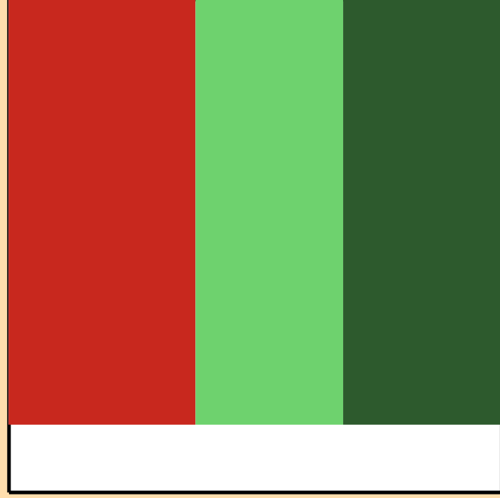
\Delta\sigma/\sigma vs. E for ^{187}\text{Tl}(n,\text{tot.})
