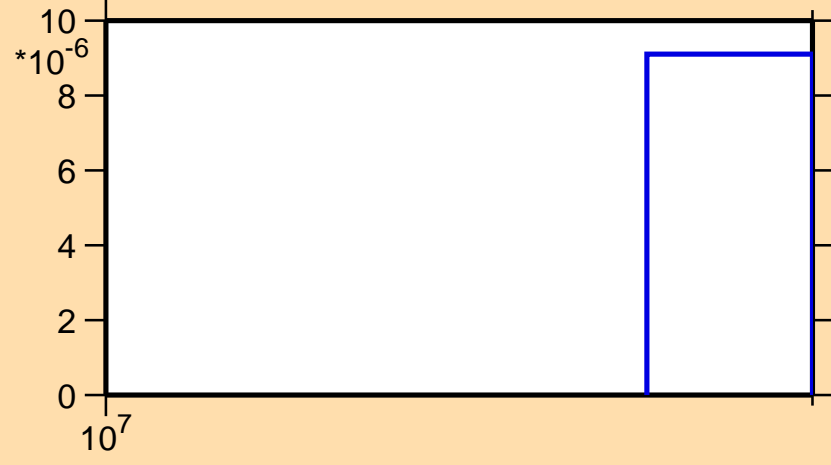
\sigma vs. E for ^{189}\text{Tl}(n,3n)
