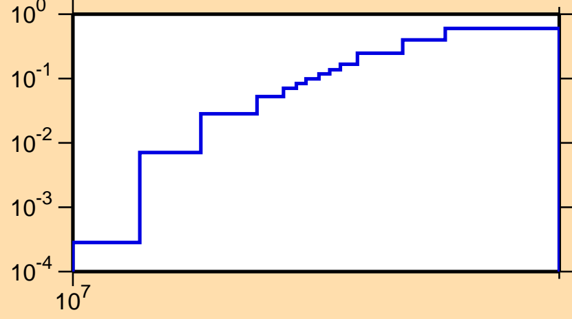
\sigma vs. E for ^{189}\text{Tl}(n,2n)
