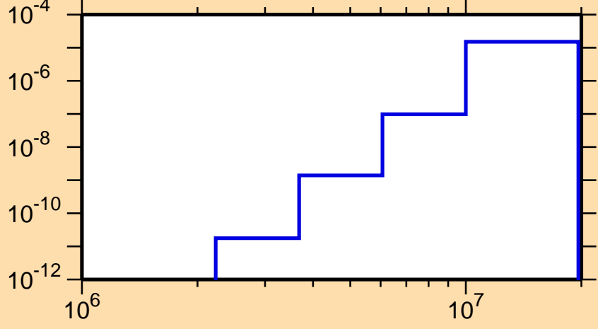
\sigma vs. E for ^{189}\text{Tl}(n,p\alpha)
