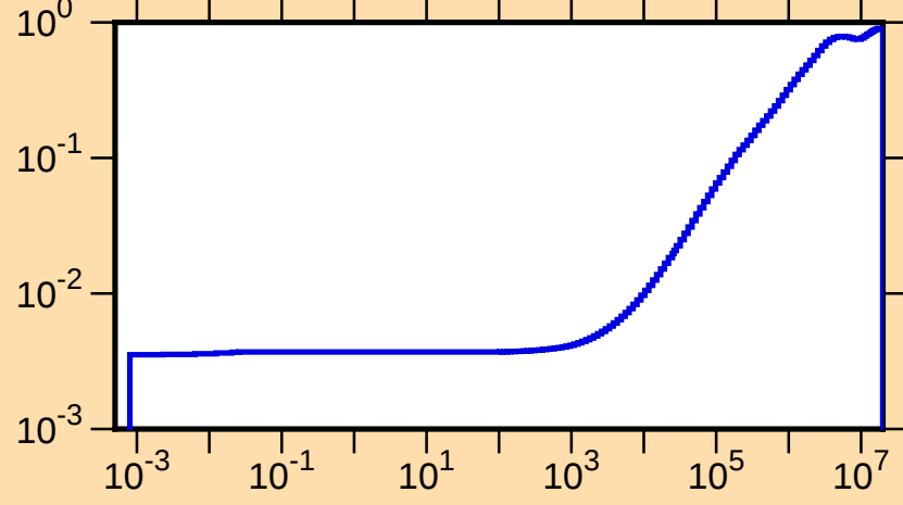
\mu vs. E for ^{191}\text{Tl}(\text{mt251})
