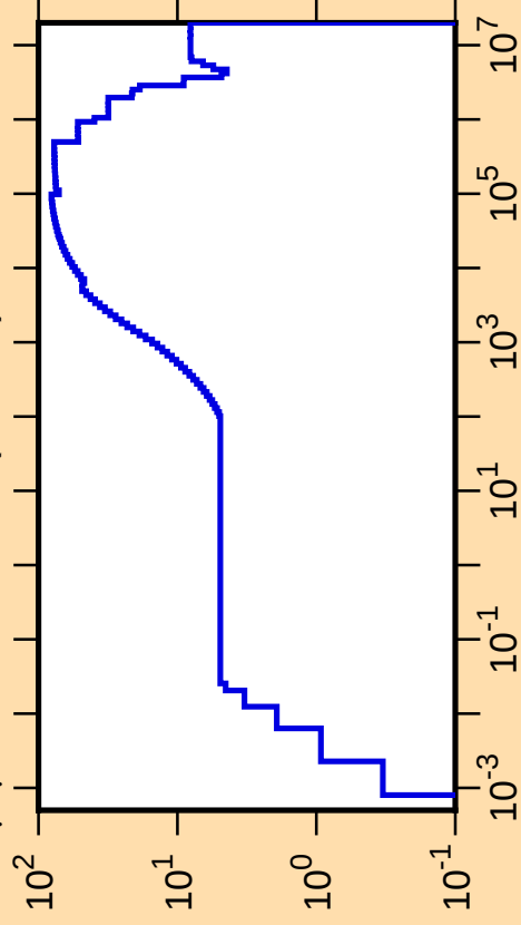
\Delta\mu/\mu vs. E for ^{191}\text{Tl}(\text{mt251})
