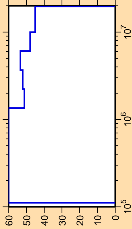
\Delta\sigma/\sigma vs. E for ^{193}\text{Tl}(n,n_3)
