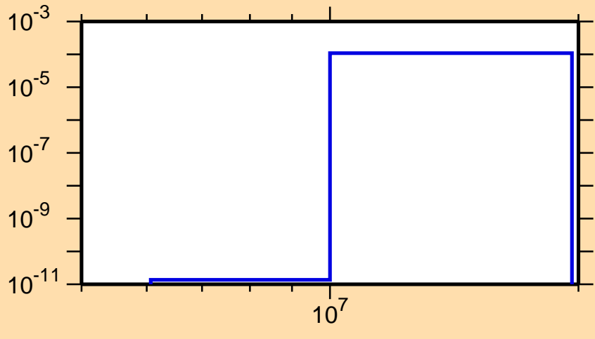
\sigma vs. E for ^{193}\text{Tl}(n,t)
