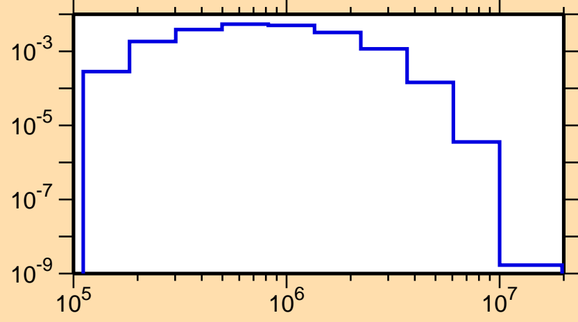
\sigma vs. E for ^{193}\text{Tl}(n,n_3)
