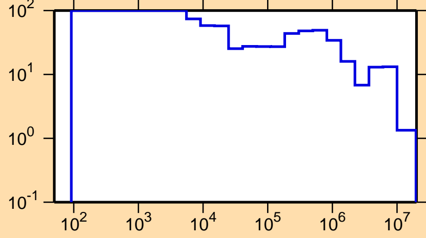
\Delta\sigma/\sigma vs. E for ^{193}\text{Tl}(n,\text{tot.})
