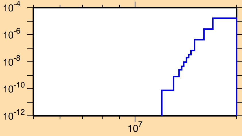
\sigma vs. E for ^{194}\text{Tl}(n,\text{nd})
