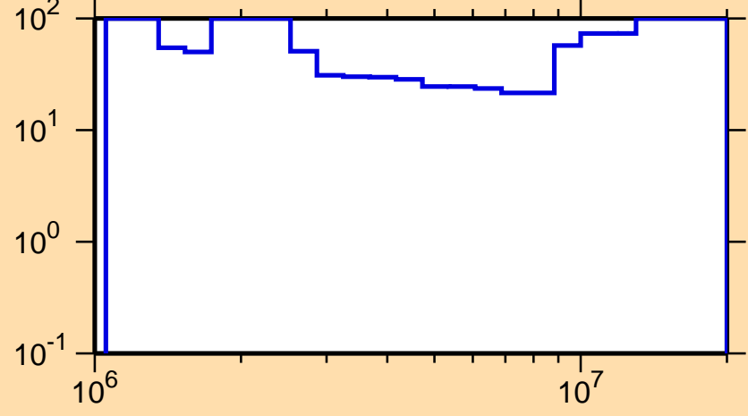
\Delta\sigma/\sigma vs. E for ^{194}\text{Tl}(n,ncont.)
