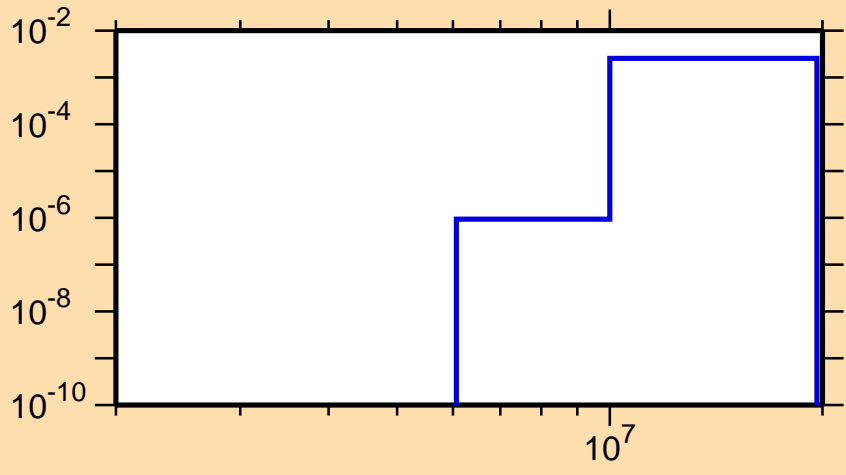
\sigma vs. E for ^{194}\text{Tl}(n,d)
