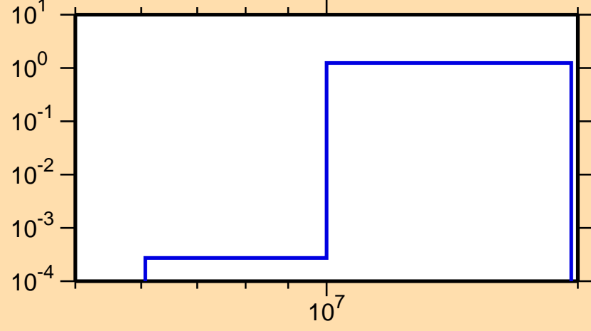
\sigma vs. E for ^{195}\text{Tl}(n,2n)
