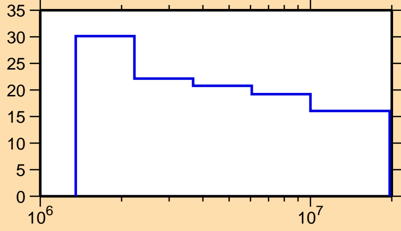
\Delta\sigma/\sigma vs. E for ^{195}\text{Tl}(n,n\text{nonel.})
