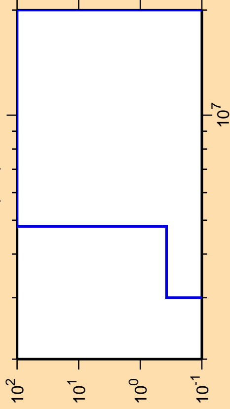
\Delta\sigma/\sigma vs. E for ^{195}\text{Tl}(n,d)
