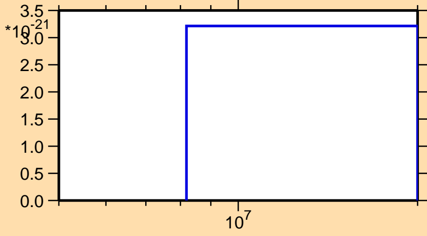
\sigma vs. E for ^{195}\text{Tl} (mt 42)
