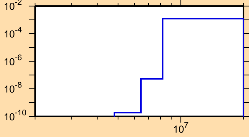
\sigma vs. E for ^{195}\text{Tl}(n,d)
