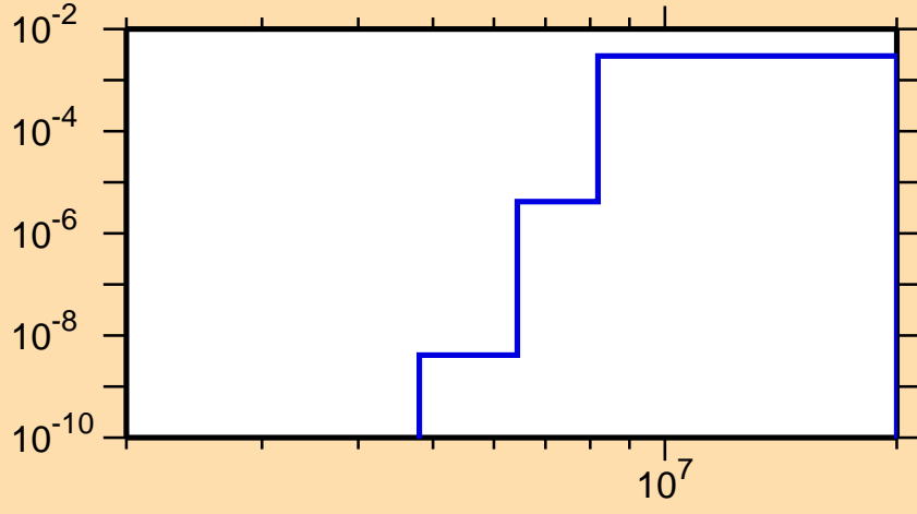
\sigma vs. E for ^{195}\text{Tl}(n,np)
