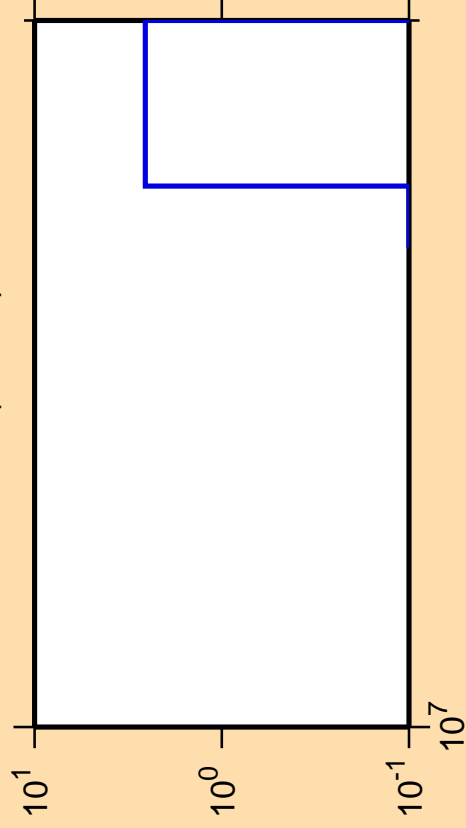
\Delta\sigma/\sigma vs. E for ^{196}\text{Tl} (mt 34)
