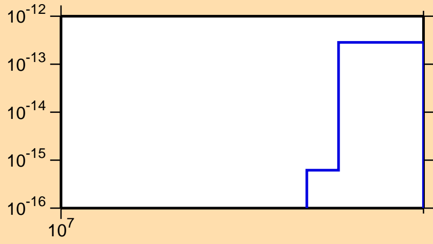
\sigma vs. E for ^{196}\text{Tl} (mt 34)
