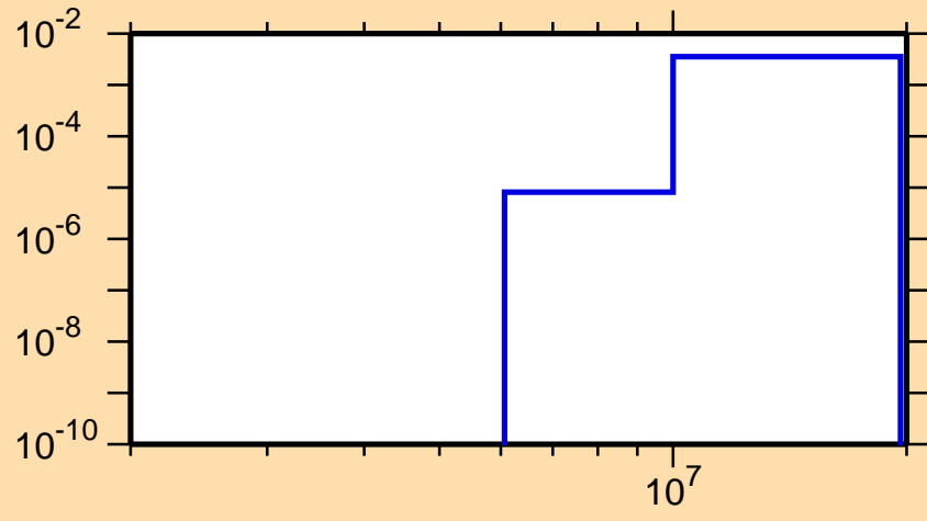
\sigma vs. E for ^{196}\text{Tl}(n,np)
