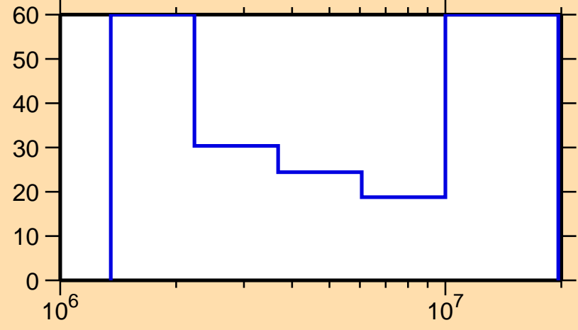
\Delta\sigma/\sigma vs. E for ^{196}\text{Tl}(n,ncont.)
