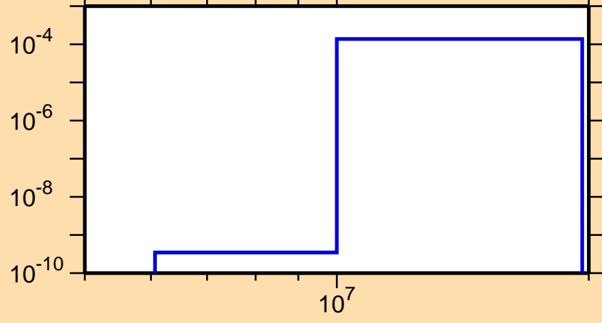
\sigma vs. E for ^{196}\text{Tl}(n,t)
