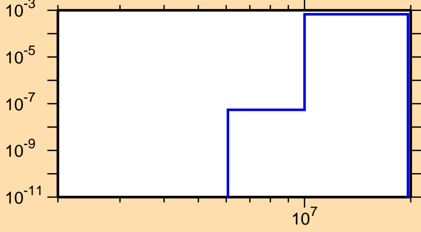
\sigma vs. E for ^{199}\text{Tl}(n,d)
