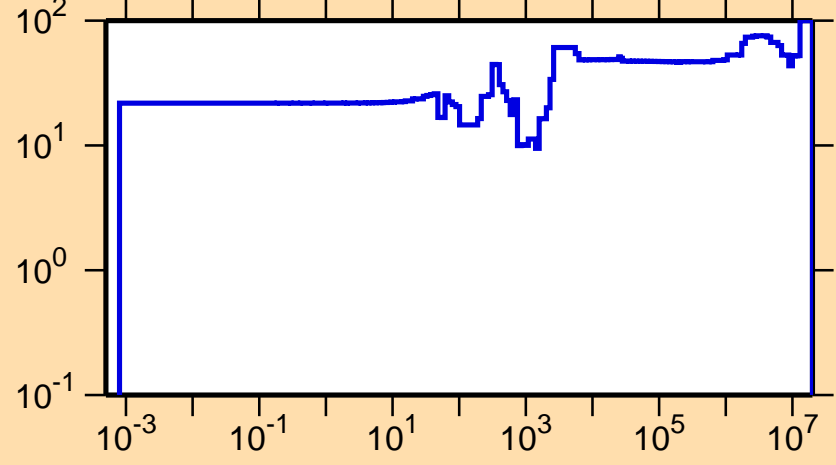
\Delta\sigma/\sigma vs. E for ^{201}\text{Tl}(n,\gamma)
