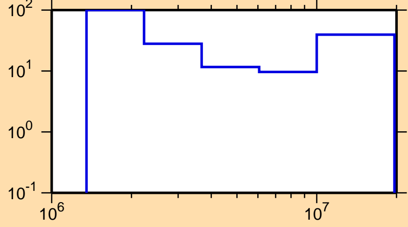
\Delta\sigma/\sigma vs. E for ^{201}\text{Tl}(n,n\text{cont.})
