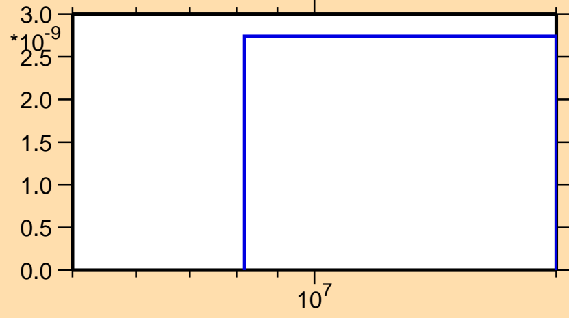
\sigma vs. E for ^{201}\text{Tl}(n,2np)
