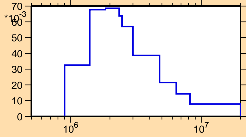
\sigma vs. E for ^{201}\text{Tl}(n,n_3)
