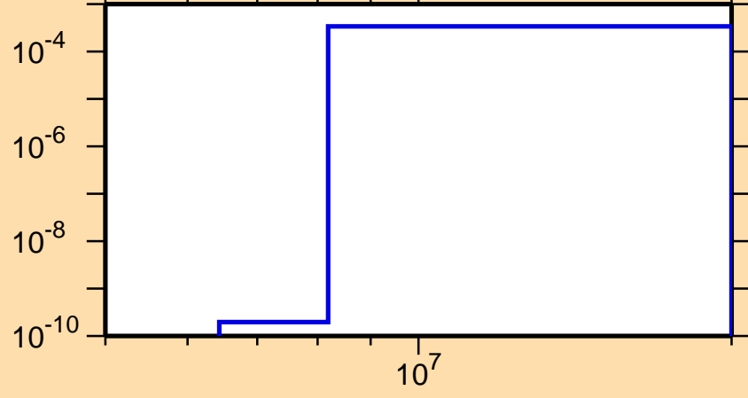
\sigma vs. E for ^{201}\text{Tl}(n,d)
