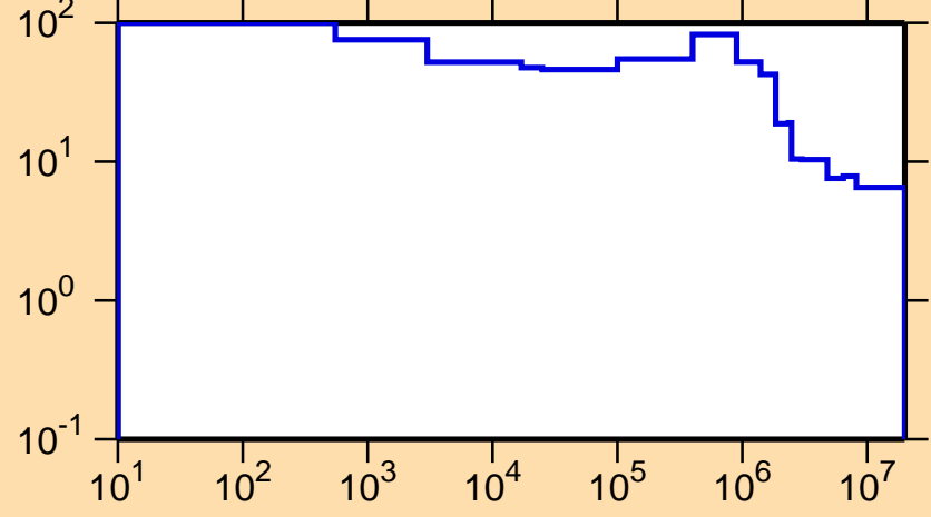
\Delta\sigma/\sigma vs. E for ^{201}\text{Tl}(n,\text{nonel.})
