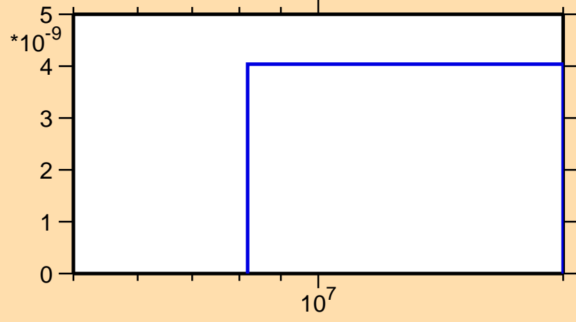
\sigma vs. E for ^{201}\text{Tl}(n,\text{nd})
