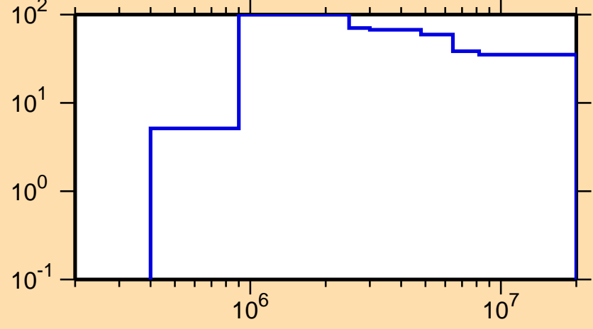
\Delta\sigma/\sigma vs. E for ^{201}\text{Tl}(n,p)
