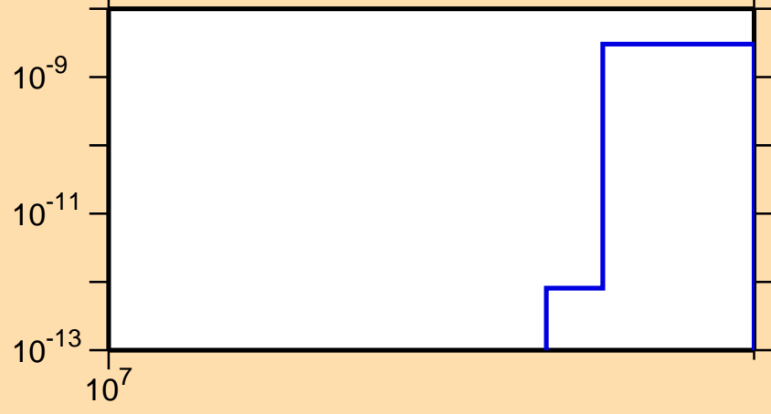
\sigma vs. E for ^{205}\text{Tl}(n,2np)
