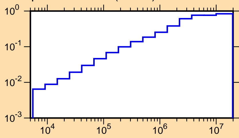
\mu vs. E for ^{205}\text{Tl}(\text{mt251})
