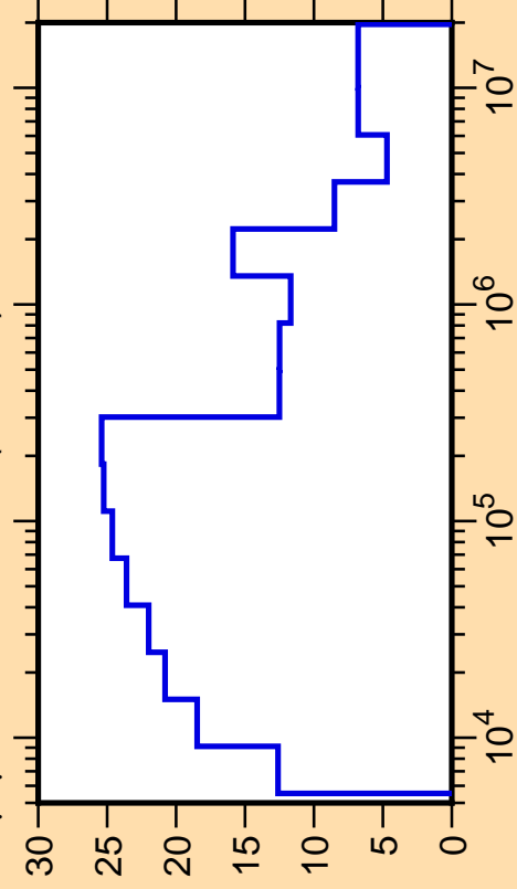
\Delta\mu/\mu vs. E for ^{205}\text{Tl}(\text{mt251})
