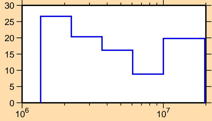
\Delta\sigma/\sigma vs. E for ^{205}\text{Tl}(n,ncont.)
