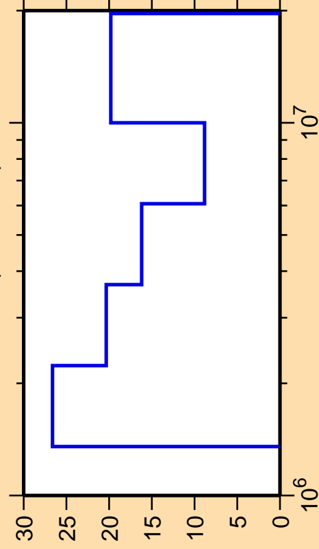
\Delta\sigma/\sigma vs. E for ^{205}\text{Tl}(n,\text{ncont.})
