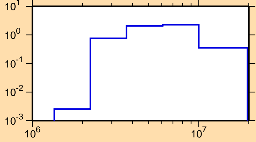
\sigma vs. E for ^{205}\text{Tl}(n,n\text{cont.})
