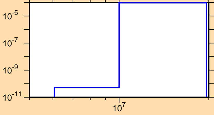
\sigma vs. E for ^{205}\text{Tl}(n,d)
