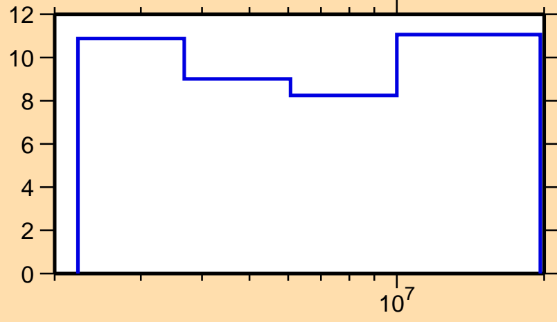
\Delta\sigma/\sigma vs. E for ^{205}\text{Tl}(n,el.)
