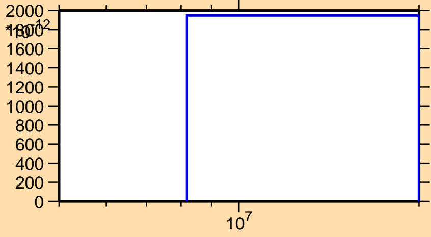
\sigma vs. E for ^{205}\text{Tl}(n,nt)
