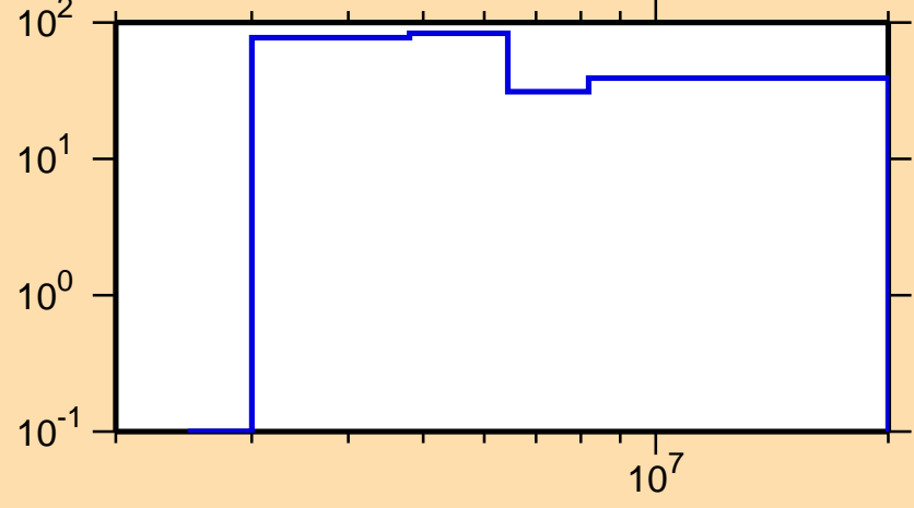
\Delta\sigma/\sigma vs. E for ^{205}\text{Tl}(n,p)
