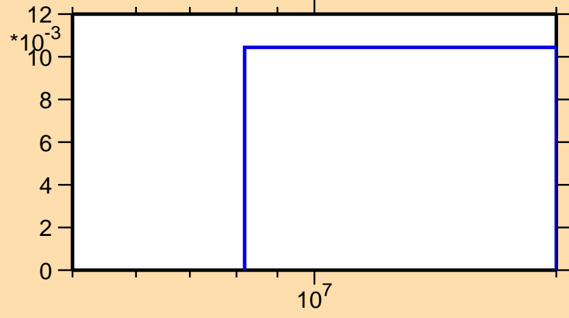
\sigma vs. E for ^{205}\text{Tl}(n,3n)
