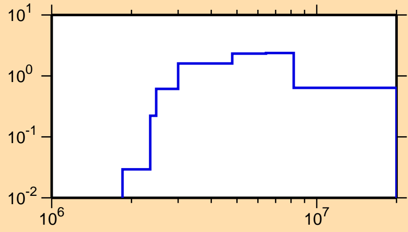
\sigma vs. E for ^{205}\text{Tl}(n,n\text{cont.})
