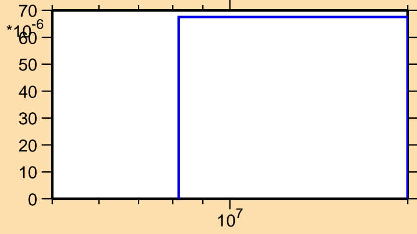
\sigma vs. E for ^{205}\text{Tl}(n,t)
