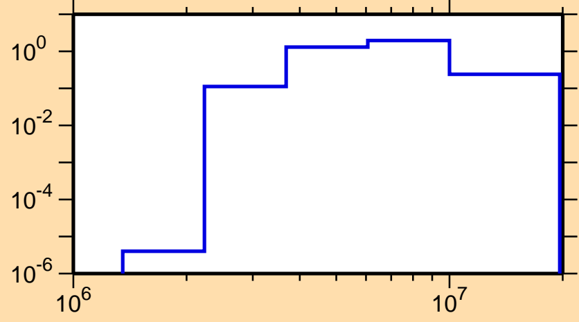
\sigma vs. E for ^{206}\text{Tl}(n,n\text{cont.})
