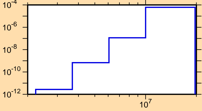
\sigma vs. E for ^{206}\text{Tl}(n,\alpha)
