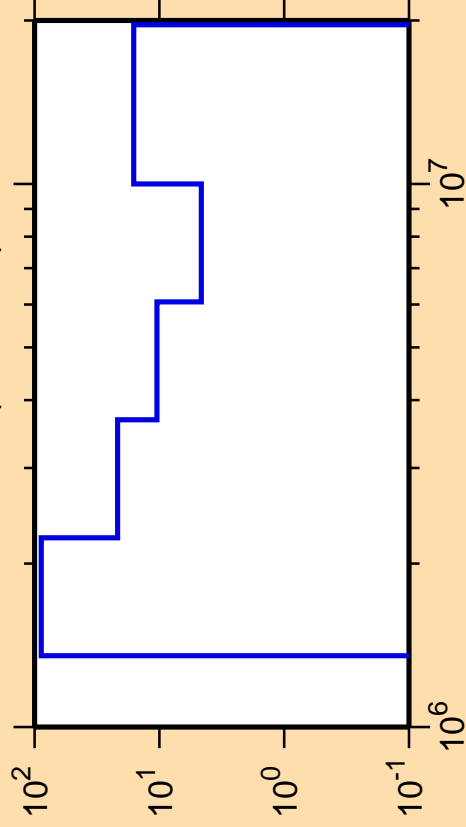
\Delta\sigma/\sigma vs. E for ^{206}\text{Tl}(n,\text{ncont.})
