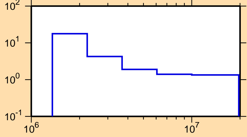
\Delta\sigma/\sigma vs. E for ^{206}\text{Tl}(n,n\text{nonel.})
