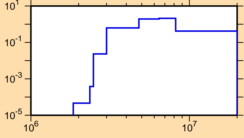
\sigma vs. E for ^{206}\text{Tl}(n,n\text{cont.})
