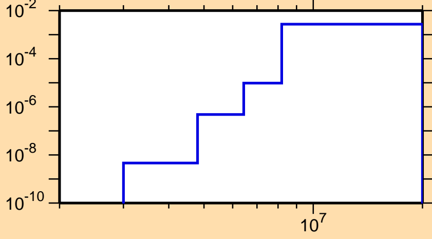
\sigma vs. E for ^{206}\text{Tl}(n,p)
