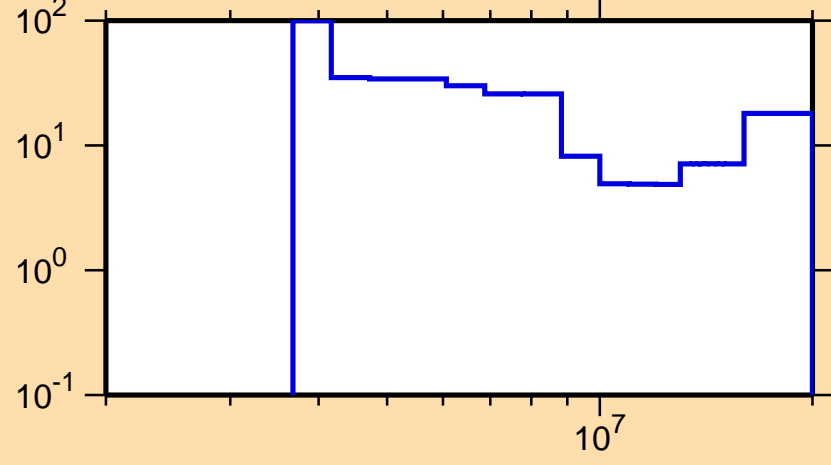
\Delta\sigma/\sigma vs. E for ^{206}\text{Tl}(n,2n)
