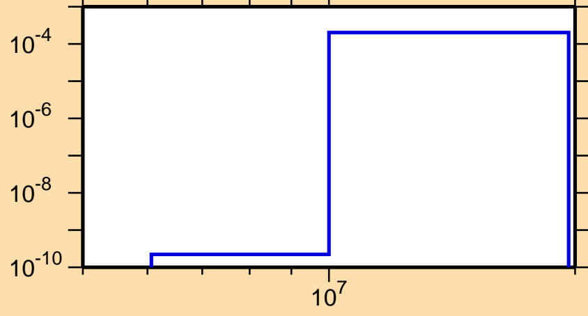
\sigma vs. E for ^{206}\text{Tl}(n,t)
