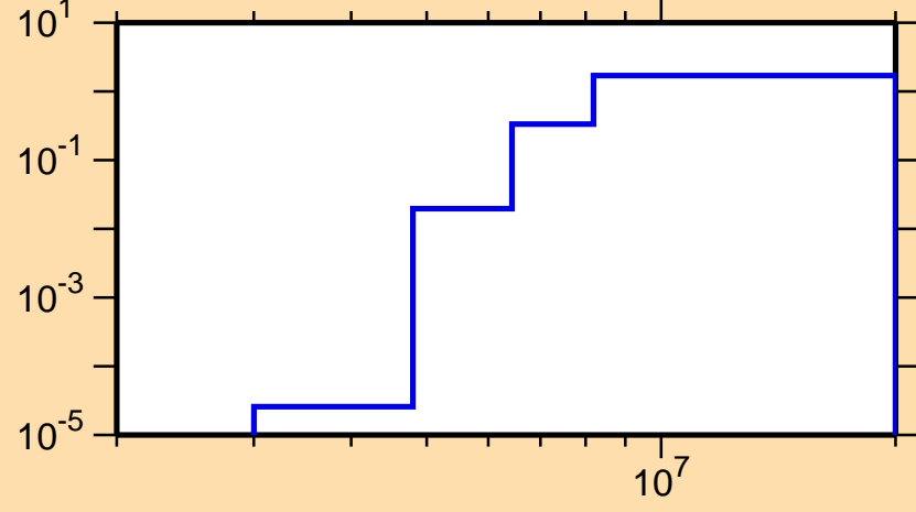
\sigma vs. E for ^{206}\text{Tl}(n,2n)
