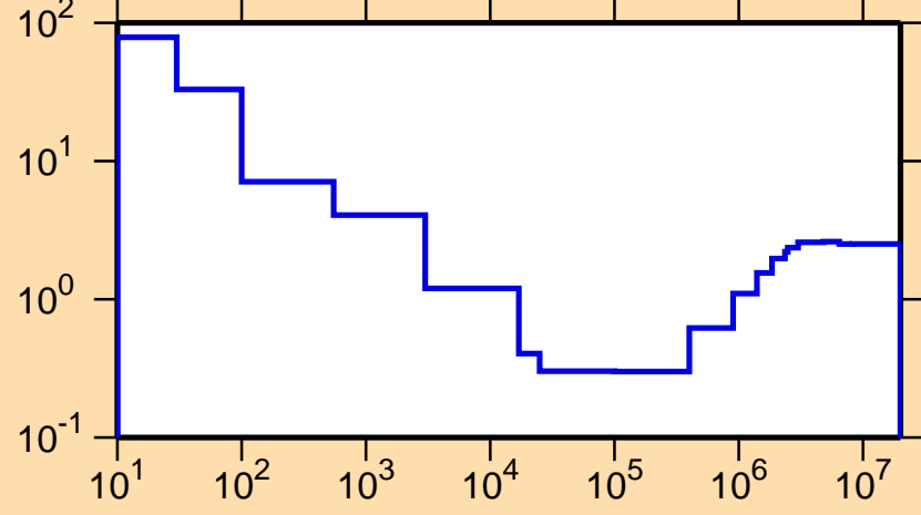
\sigma vs. E for ^{206}\text{Tl}(n,\text{nonel.})
