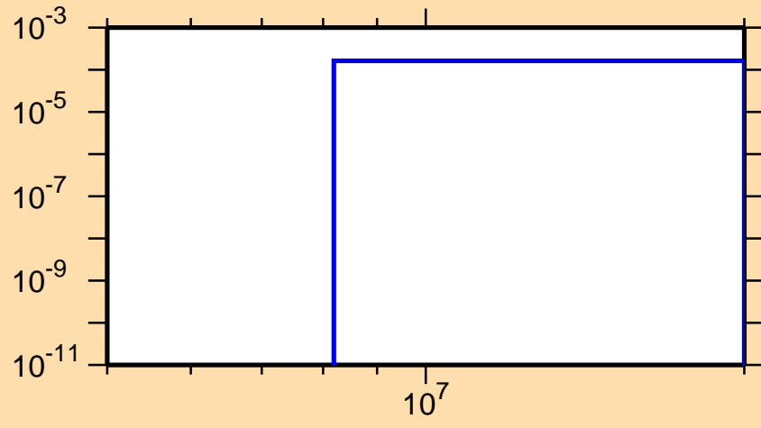
\sigma vs. E for ^{206}\text{Tl}(n,t)
