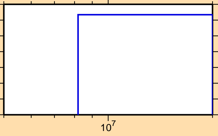
\sigma vs. E for ^{206}\text{Tl}(n,\text{nd})
