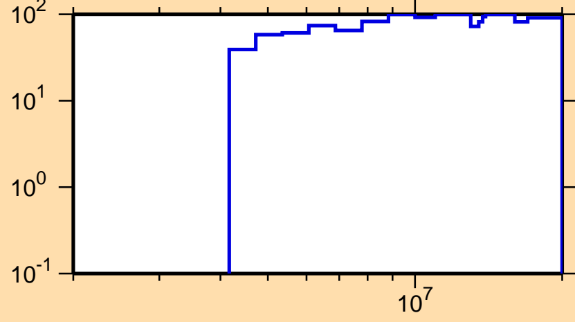
\Delta\sigma/\sigma vs. E for ^{207}\text{Tl}(n,n_1)
