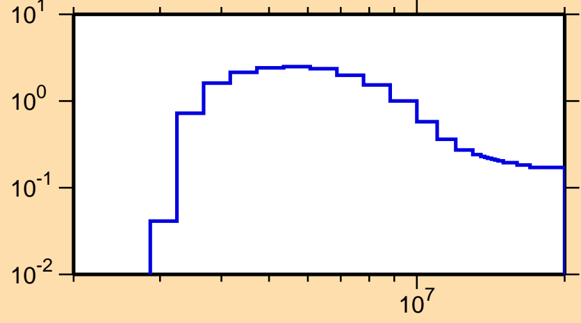
\sigma vs. E for ^{207}\text{Tl}(n,n\text{cont.})
