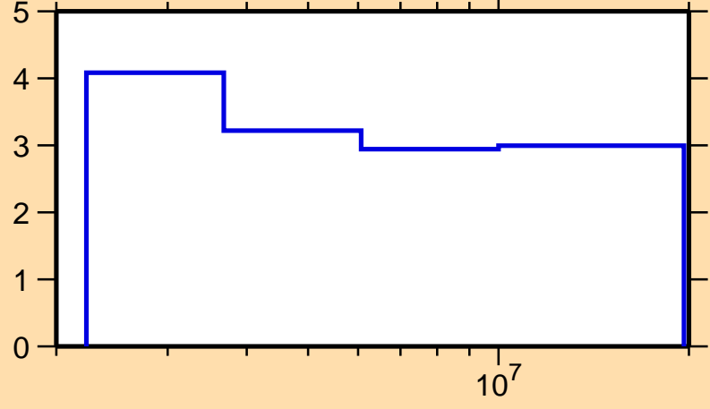
\Delta\sigma/\sigma vs. E for ^{207}\text{Tl}(n,n\text{nonel.})
