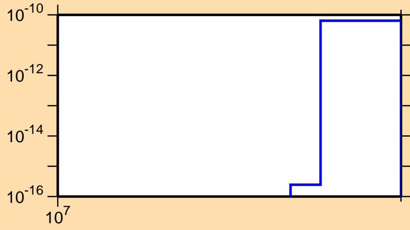
\sigma vs. E for ^{210}\text{Tl} (mt 11)
