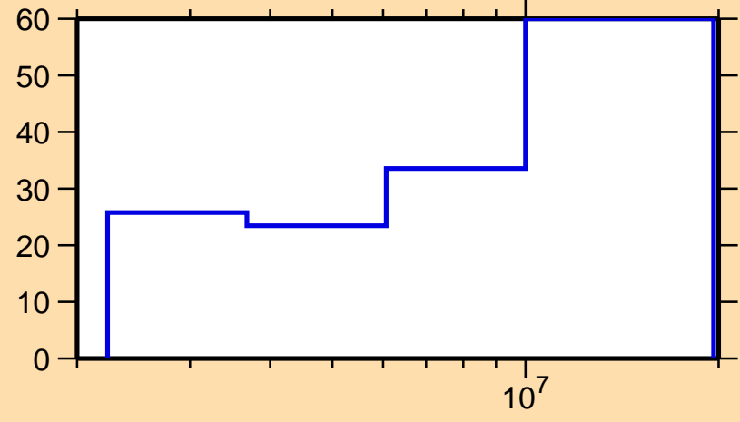
\Delta\sigma/\sigma vs. E for ^{210}\text{Tl}(n,n\text{cont.})
