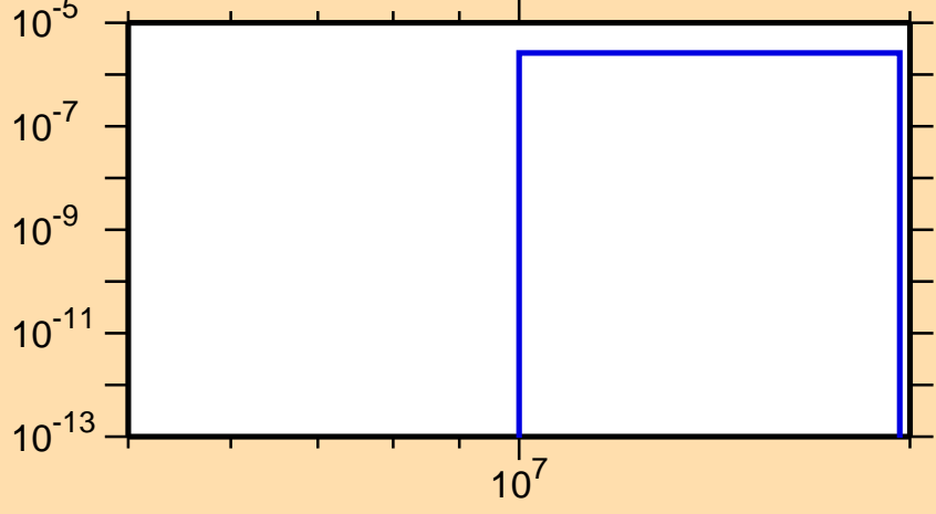
\sigma vs. E for ^{210}\text{Tl}(n,nt)
