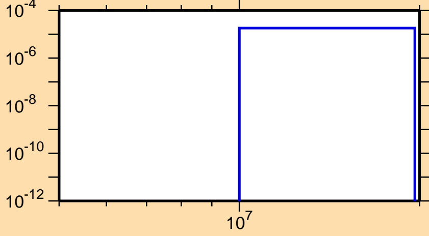
\sigma vs. E for ^{210}\text{Tl}(n,np)
