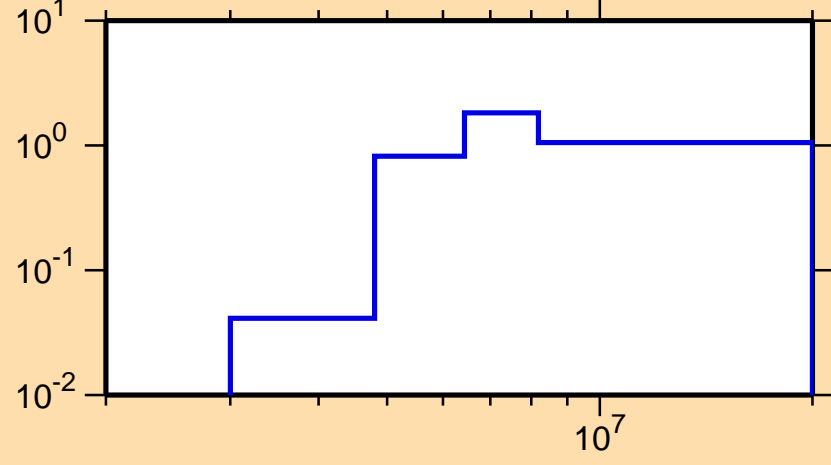
\sigma vs. E for ^{210}\text{Tl}(n,2n)
