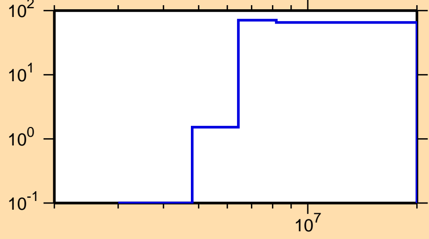
\Delta\sigma/\sigma vs. E for ^{210}\text{Tl}(n,p)
