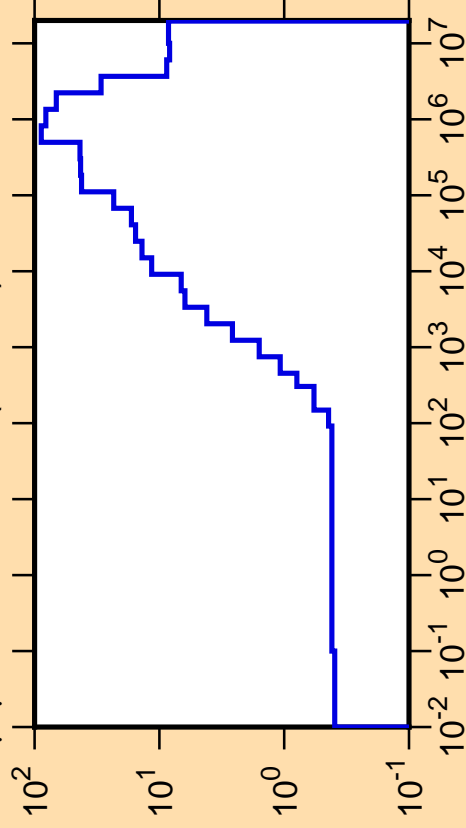
\Delta\mu/\mu vs. E for ^{216}\text{Tl}(\text{mt251})
