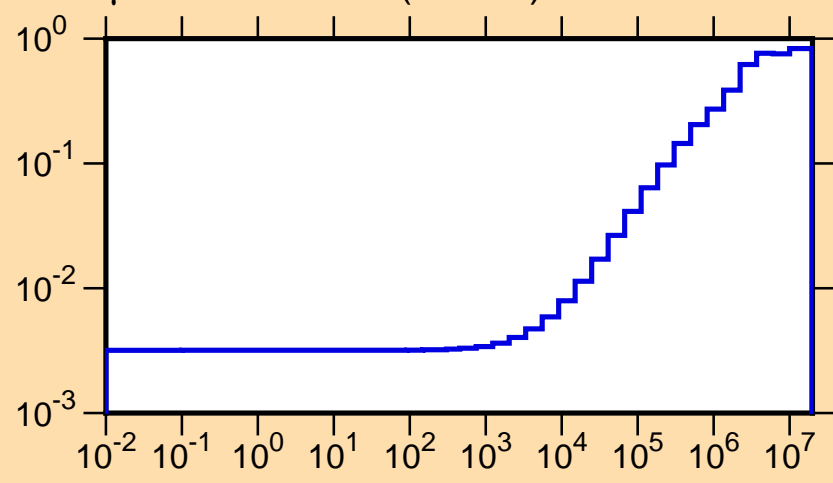
\mu vs. E for ^{216}\text{Tl}(\text{mt251})
