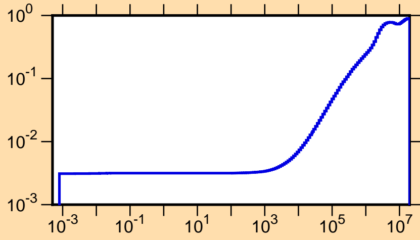
\mu vs. E for ^{217}\text{Tl}(\text{mt251})
