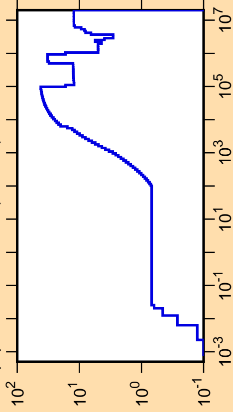
\Delta\mu/\mu vs. E for ^{217}\text{Tl}(\text{mt251})
